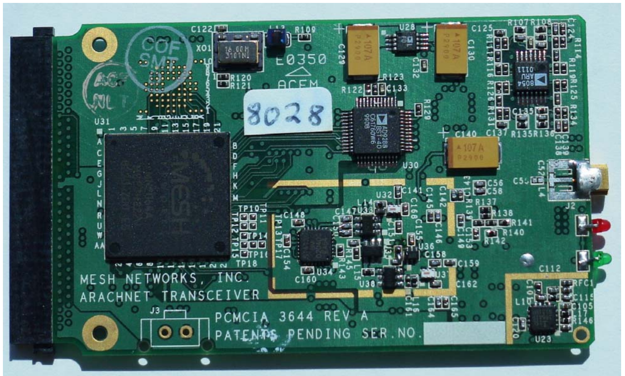
MWR6300 PCMCIA Top Side
