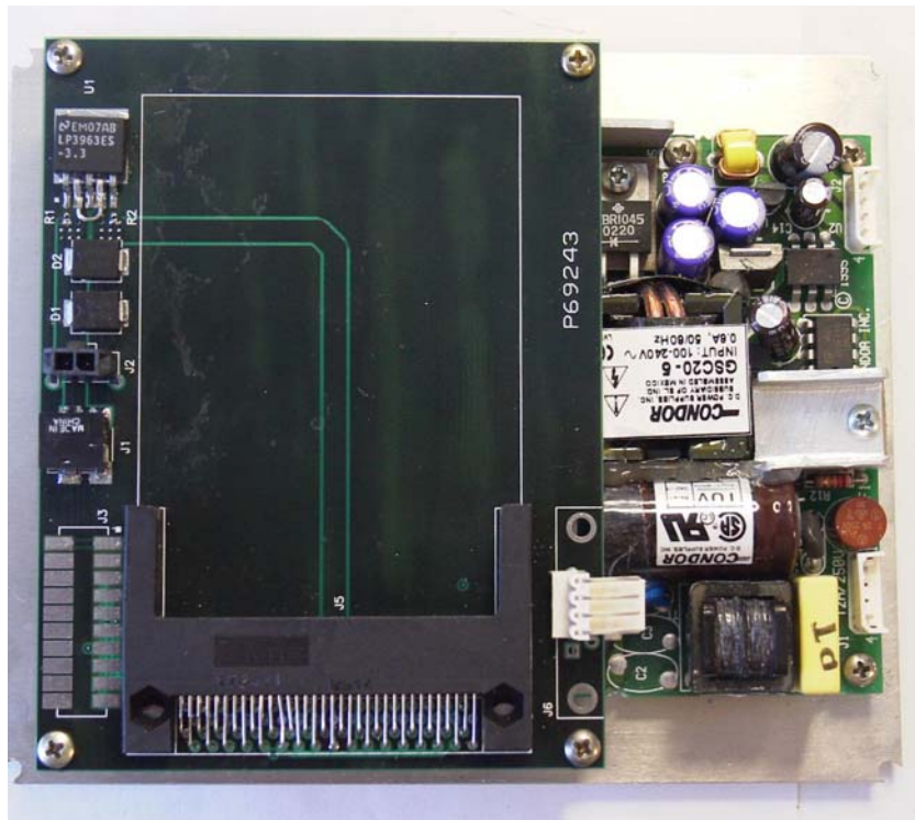
MWR6300 PCMCIA Adapter card & Power Supply
