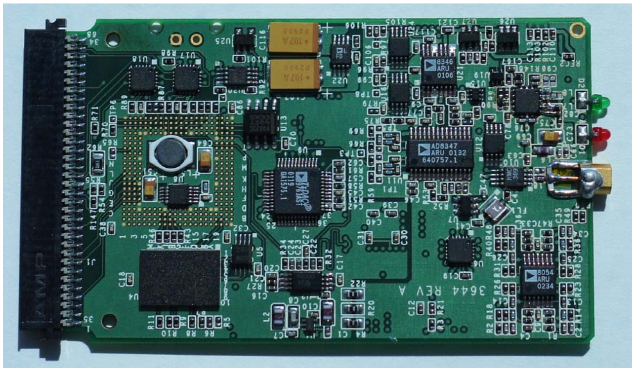
MWR6300 PCMCIA Bottom Side
