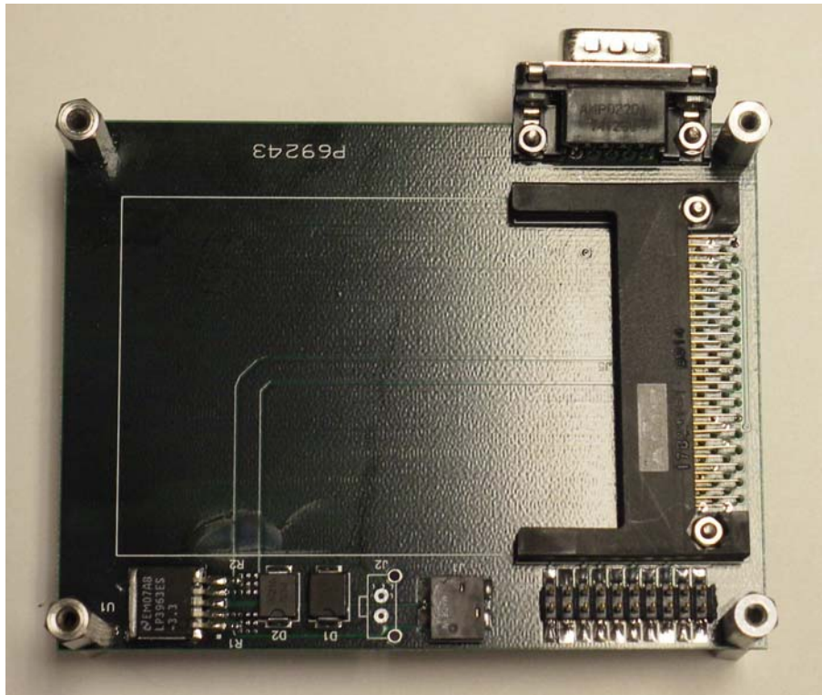
MWR6300 PCMCIA Adapter Card Top Side
