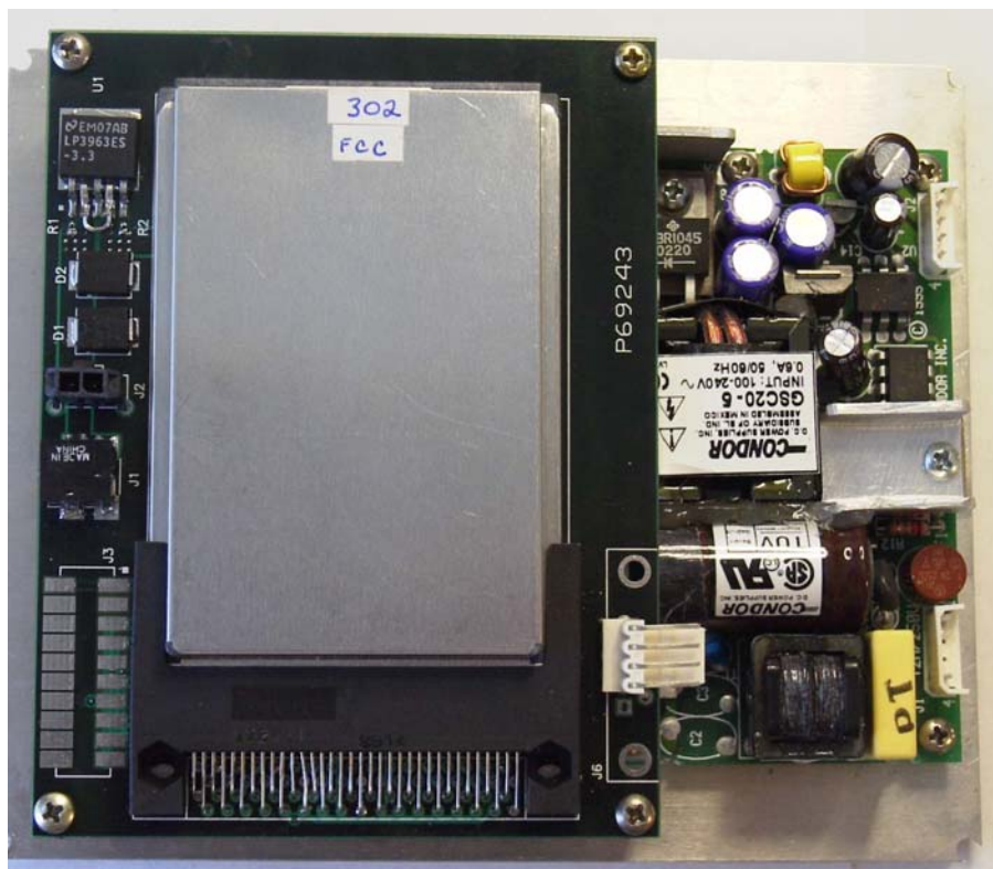
MWR6300 PCMCIA Adapter card & Power Supply with PCMCIA Card
