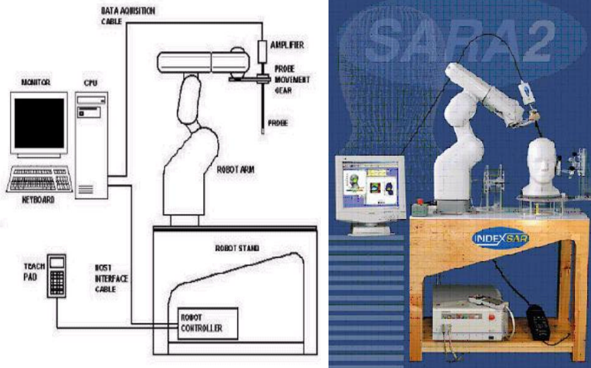
Figure 9. Block Diagram of SARA 2 System
