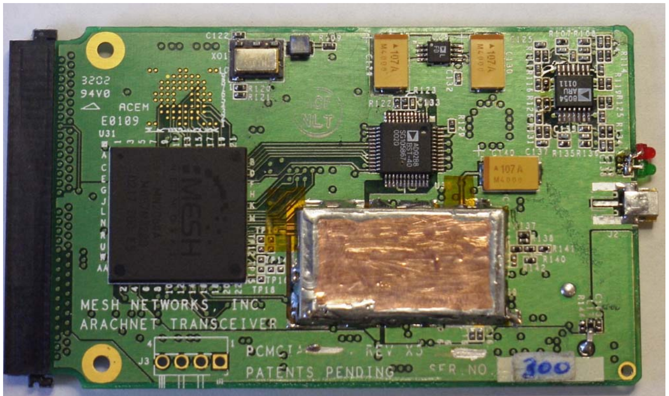
WMC6300 PCMCIA Top Side
