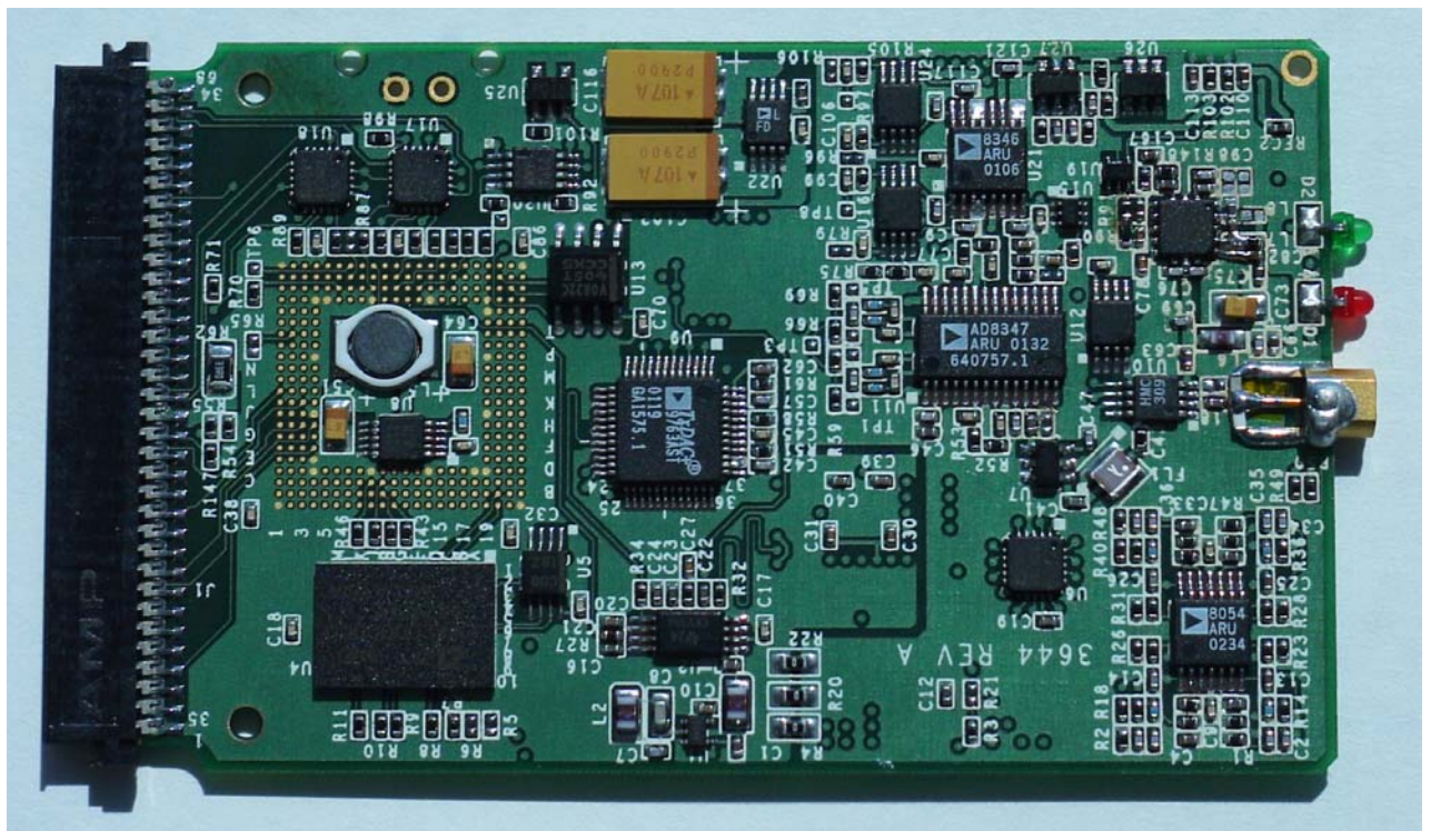
WMC6300 PCMCIA Bottom Side
