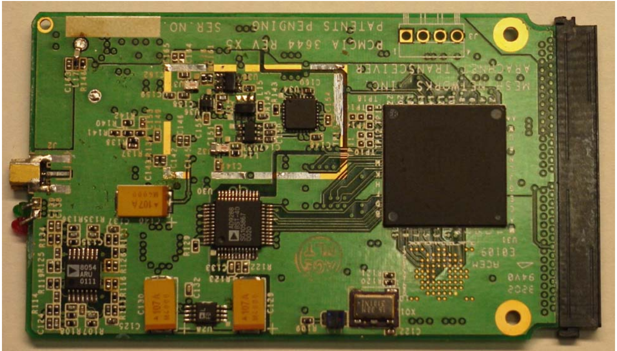
WMC6300 PCMCIA Top Side – No Shield
