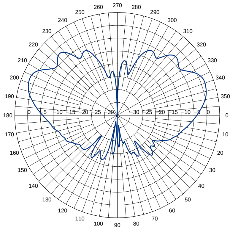
BMMG2400 Elevation Cut
