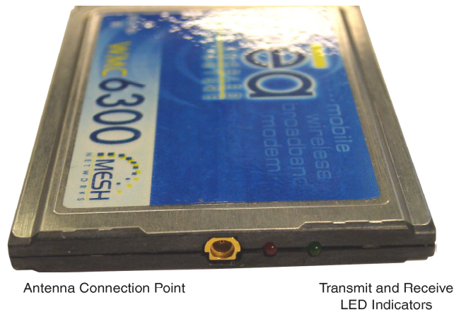
Figure 3. WMC6300 Antenna Port and LED Indicators
