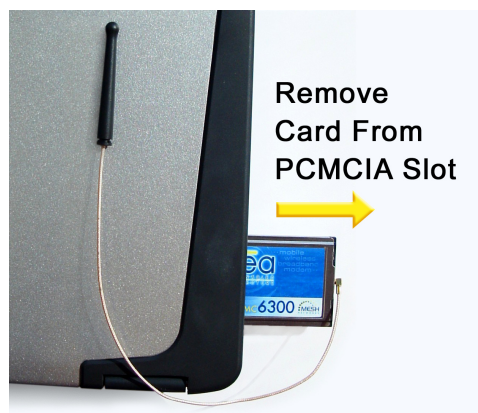
Figure 18. Removing the WMC6300 from the PCMCIA slot
