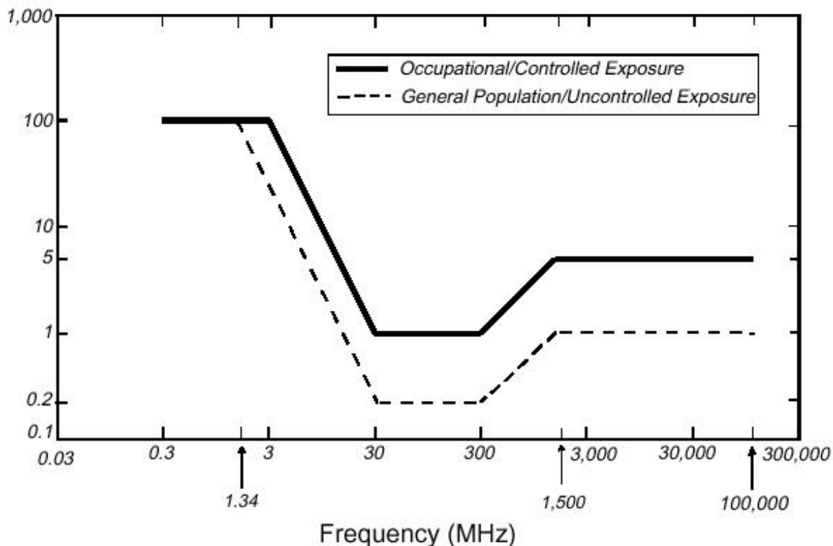
Figure A-1: FCC limits for maximum permissible exposure (MPE) plane-wave equivalent power density \text{mW/cm}^2 .
