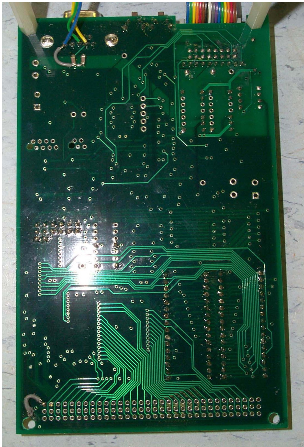
Foil Side/PCB2
