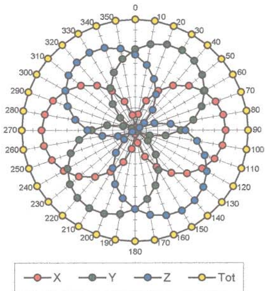
f = 1800 MHz, WG R22
