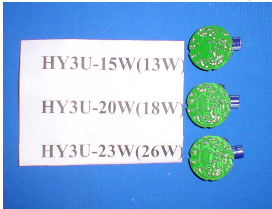
Figure 4 M/N: HY3U Series Main Board, Soldered Side
