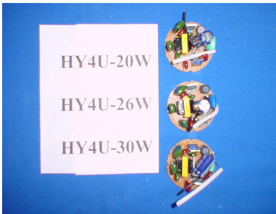
Figure 7 M/N: HY4U Series Main Board, Component Side
