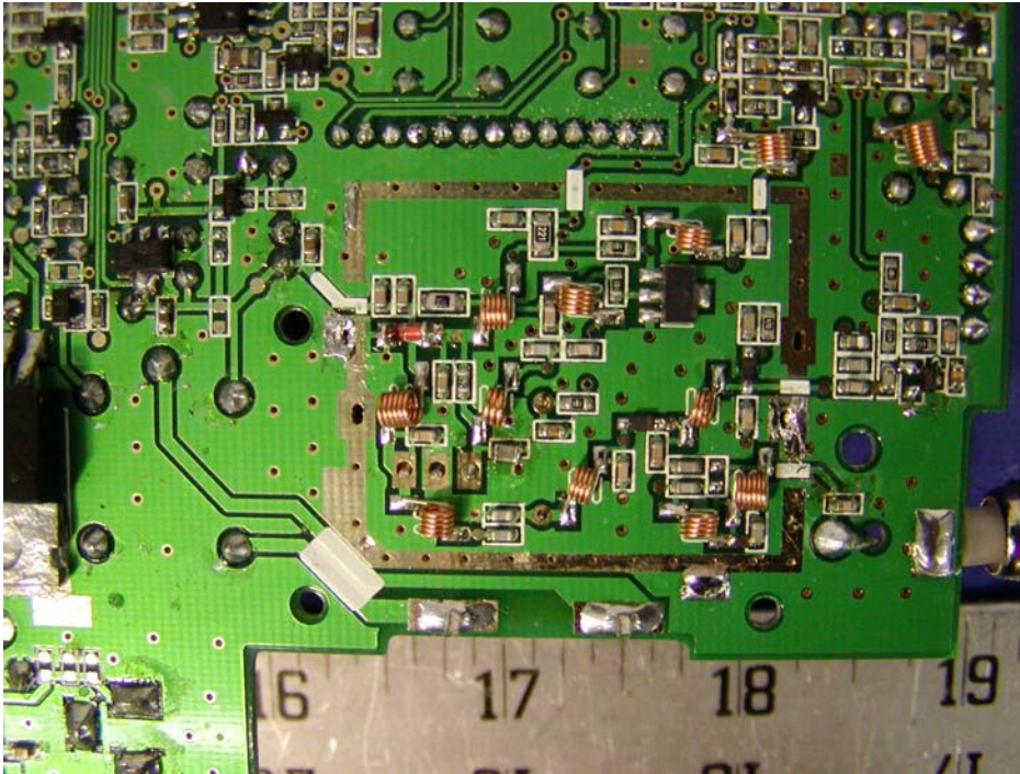
Transceiver - Component View
