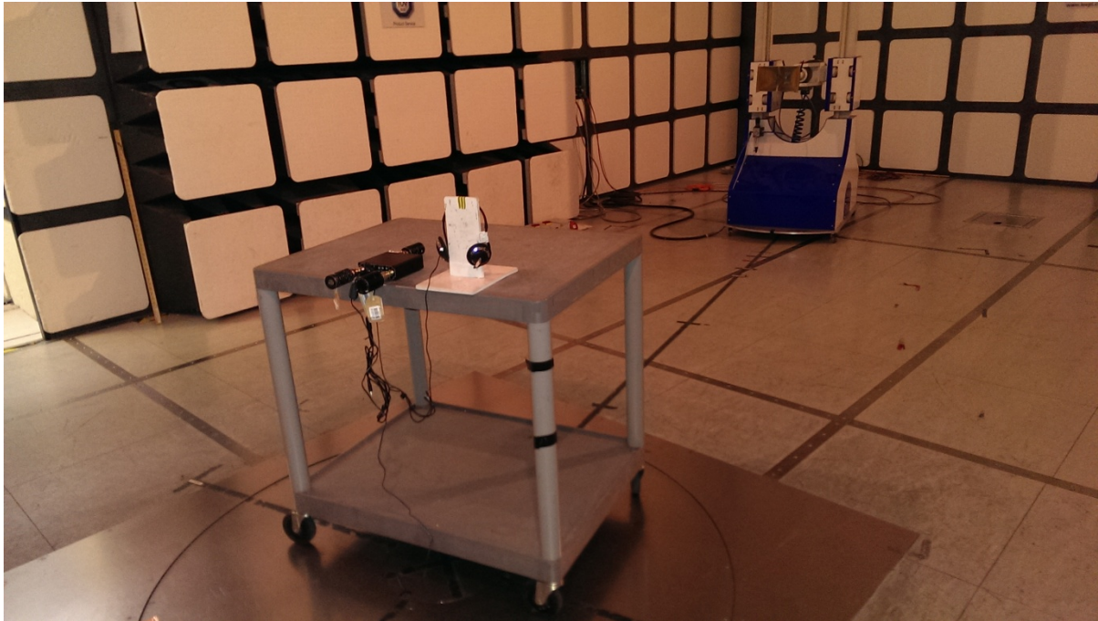
Radiated Emissions 1-2GHz
