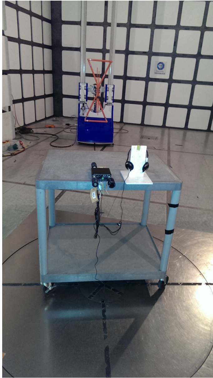
Radiated Emissions 30MHz-1GHz
