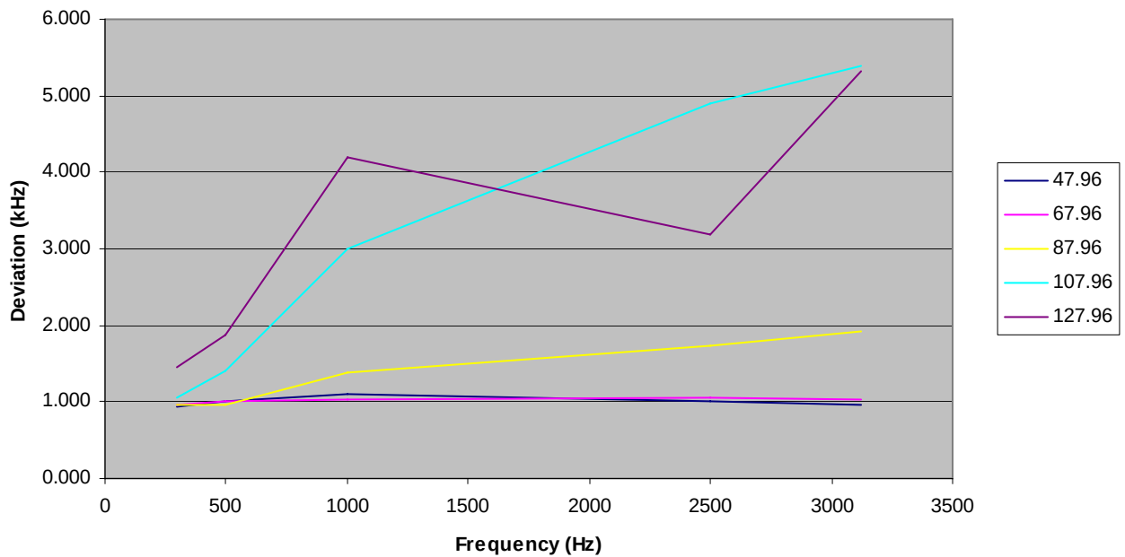
Modulation Limiting Characteristics over frequency with fixed voltage (dBmV)
