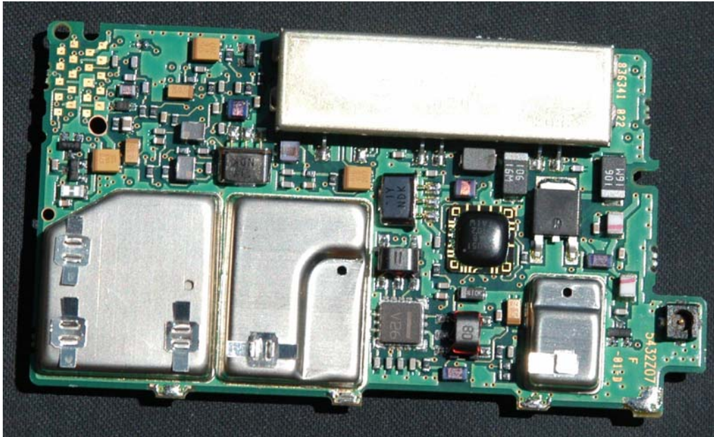
Transceiver board
