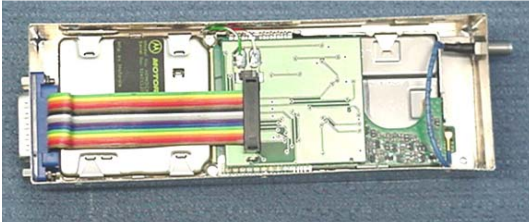
Internal view
