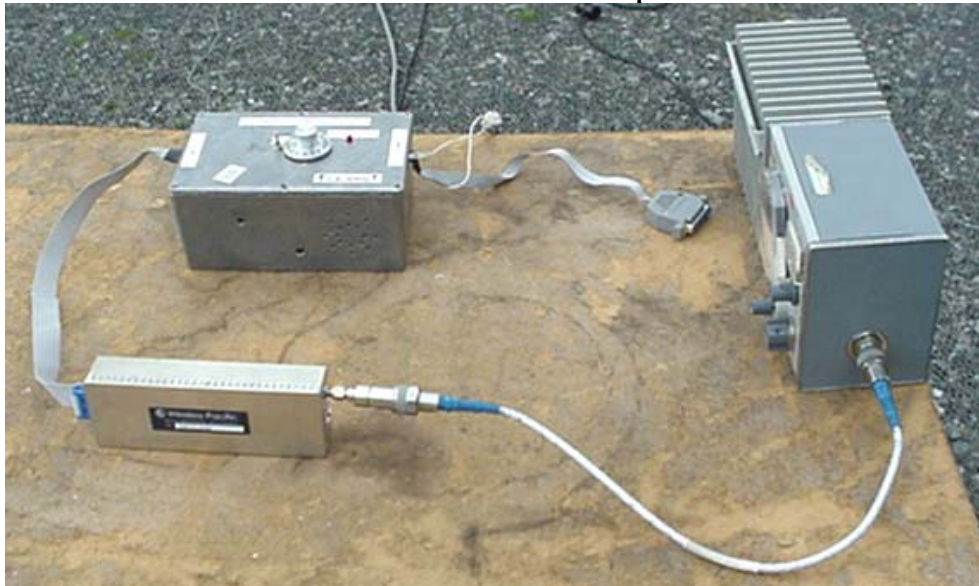
Radiated emission test set up
