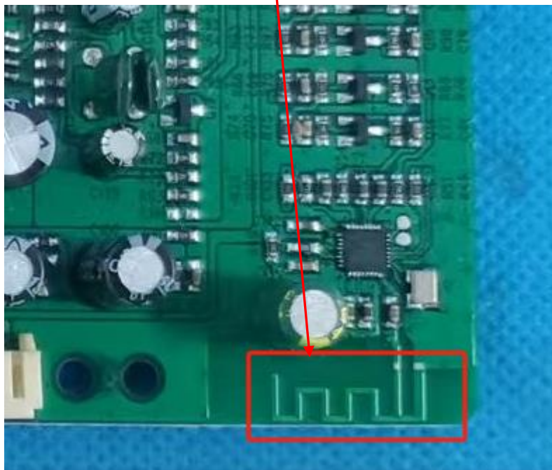
View of wireless antenna
