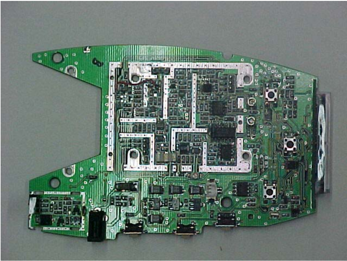
Shielding removed
