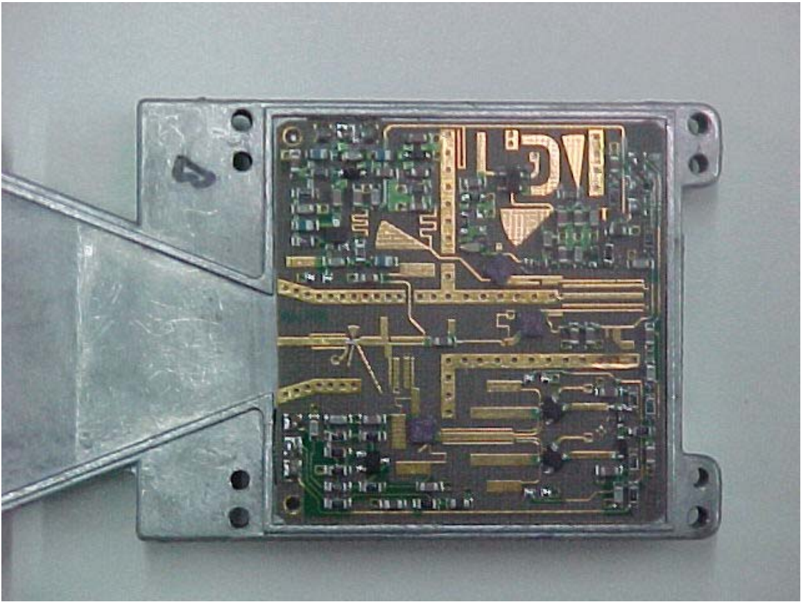
Board removed
