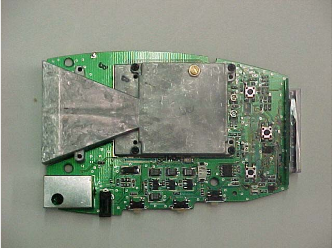
Top of Board
