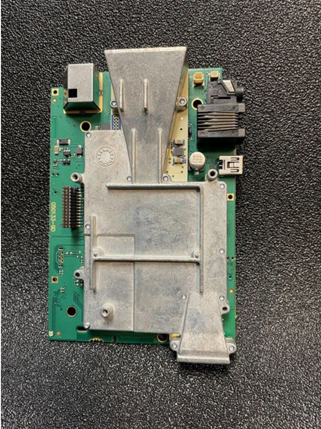
Main Board Top with Laser Shield
