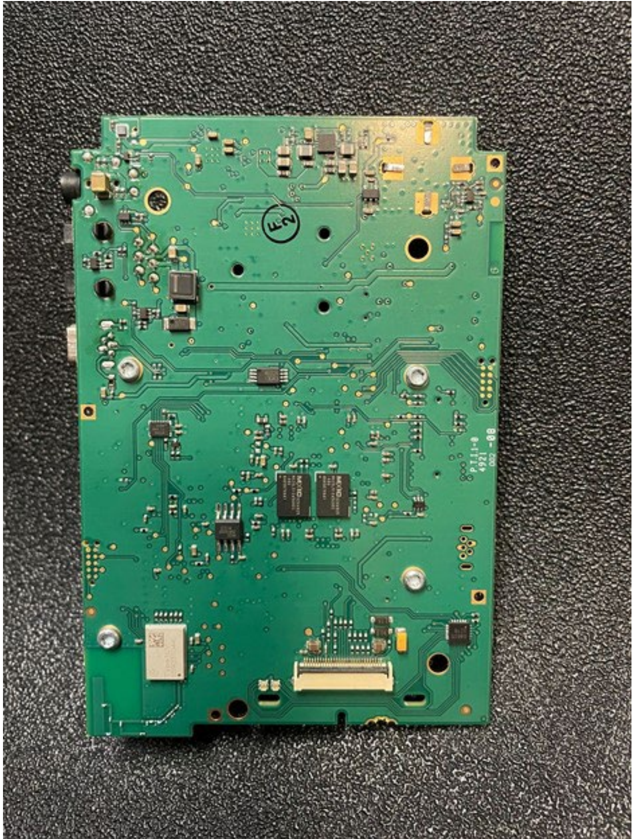
Main Board Bottom
