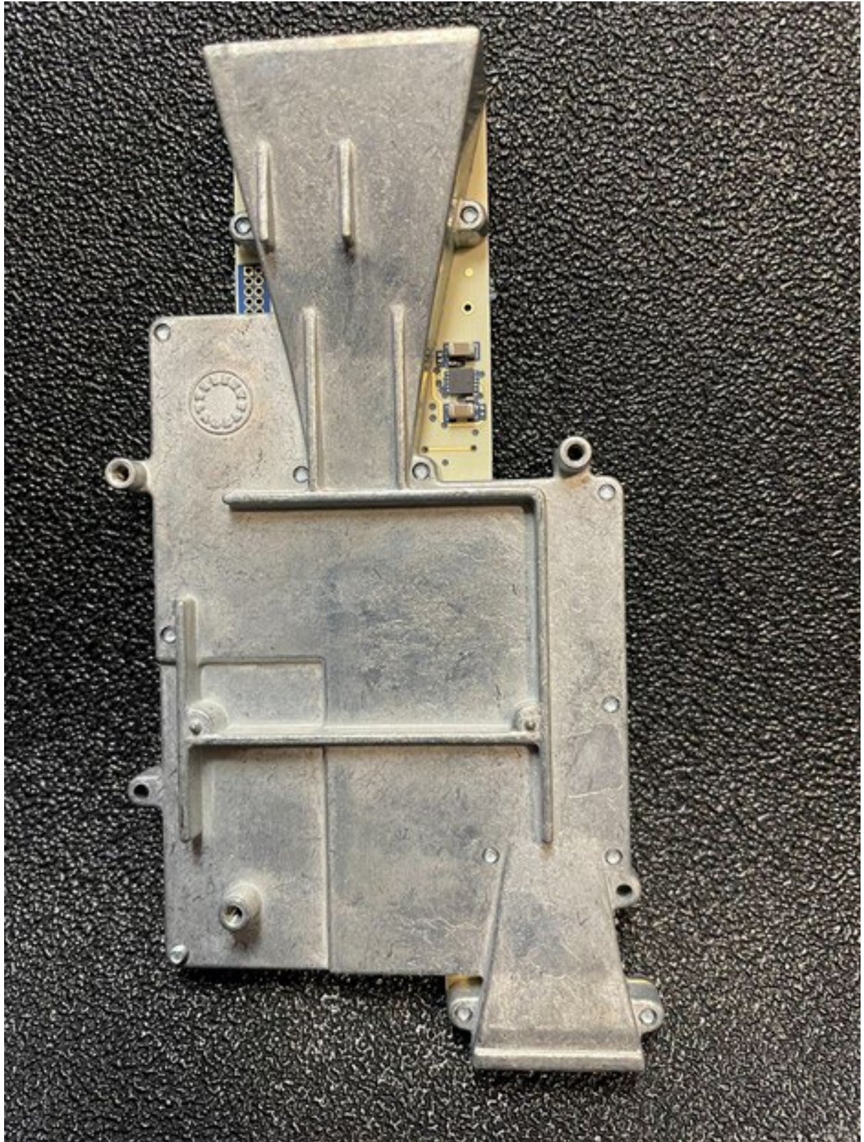
Antenna top with horn
