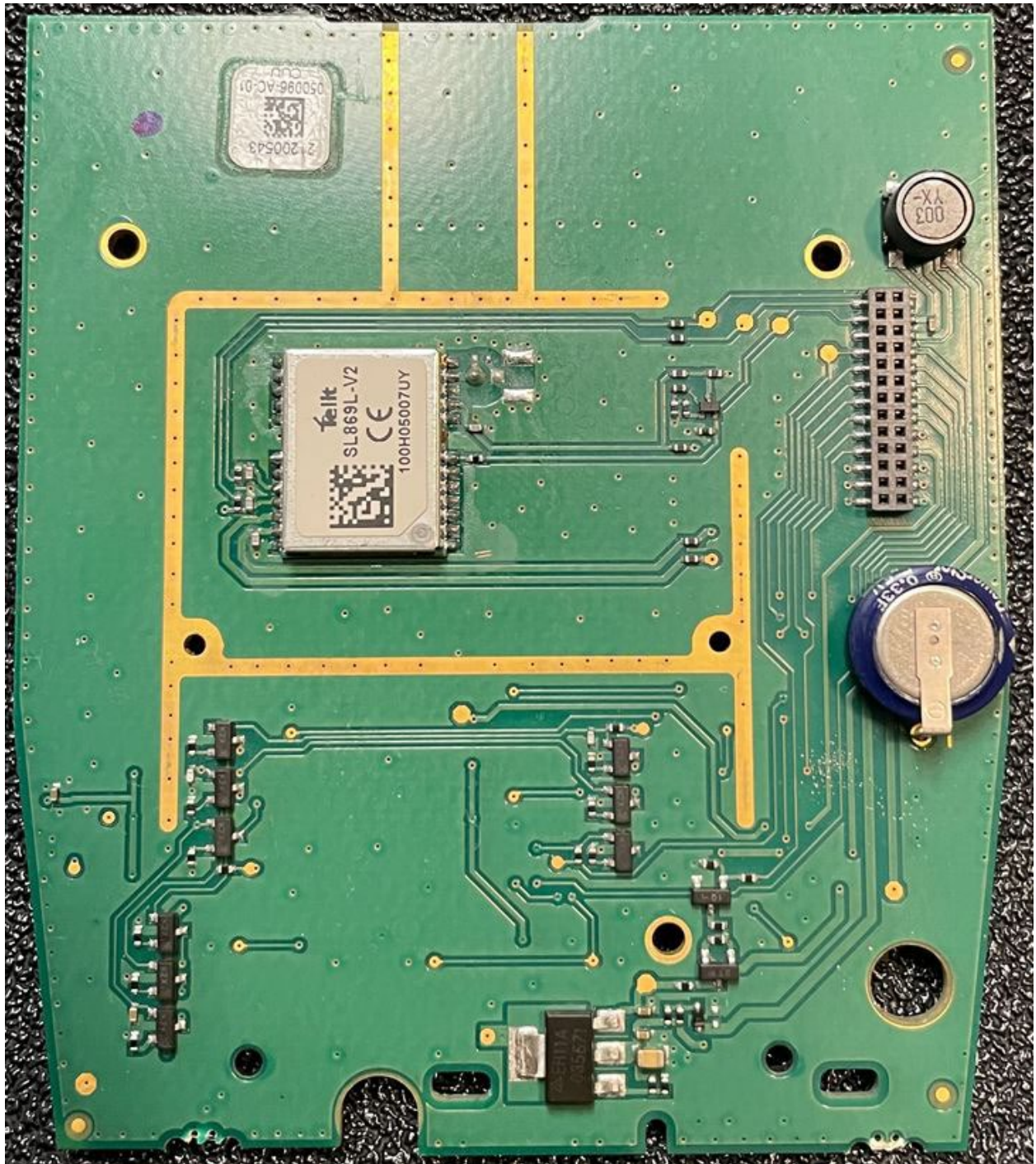
GPS BOTTOM VIEW
