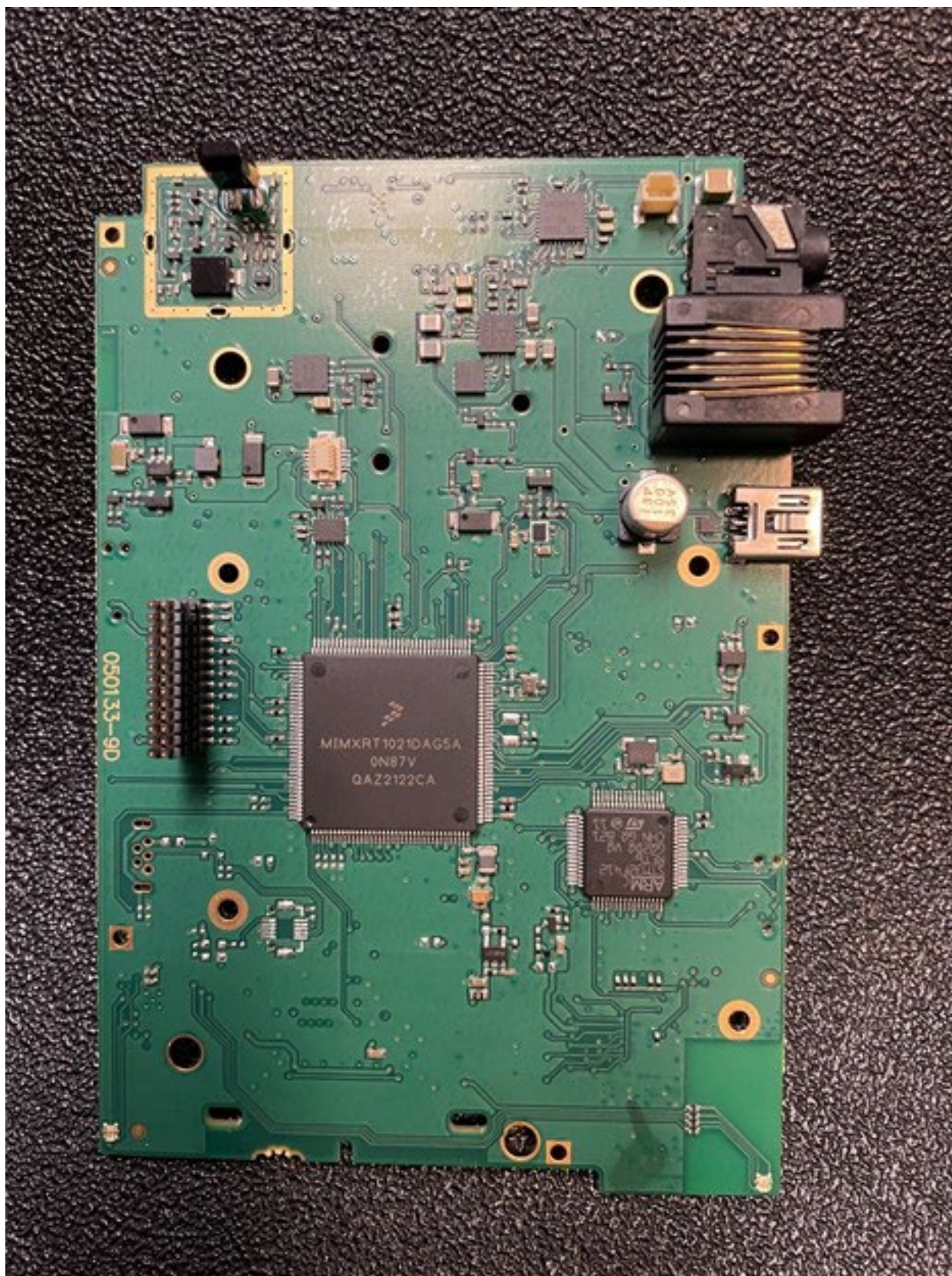
Main Board – Top no laser shield
