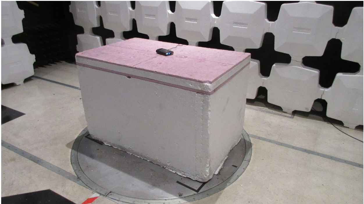
Radiated Testing, Table Setup #1
