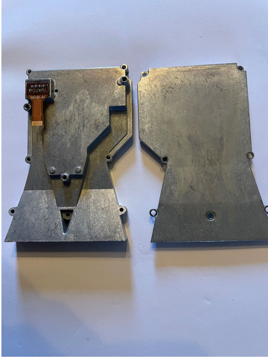
Feedhorn External Assembly
