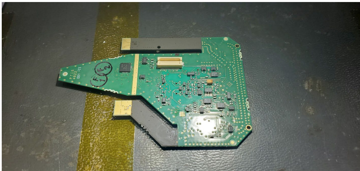
Internal Feedhorn PCB Bottom View
