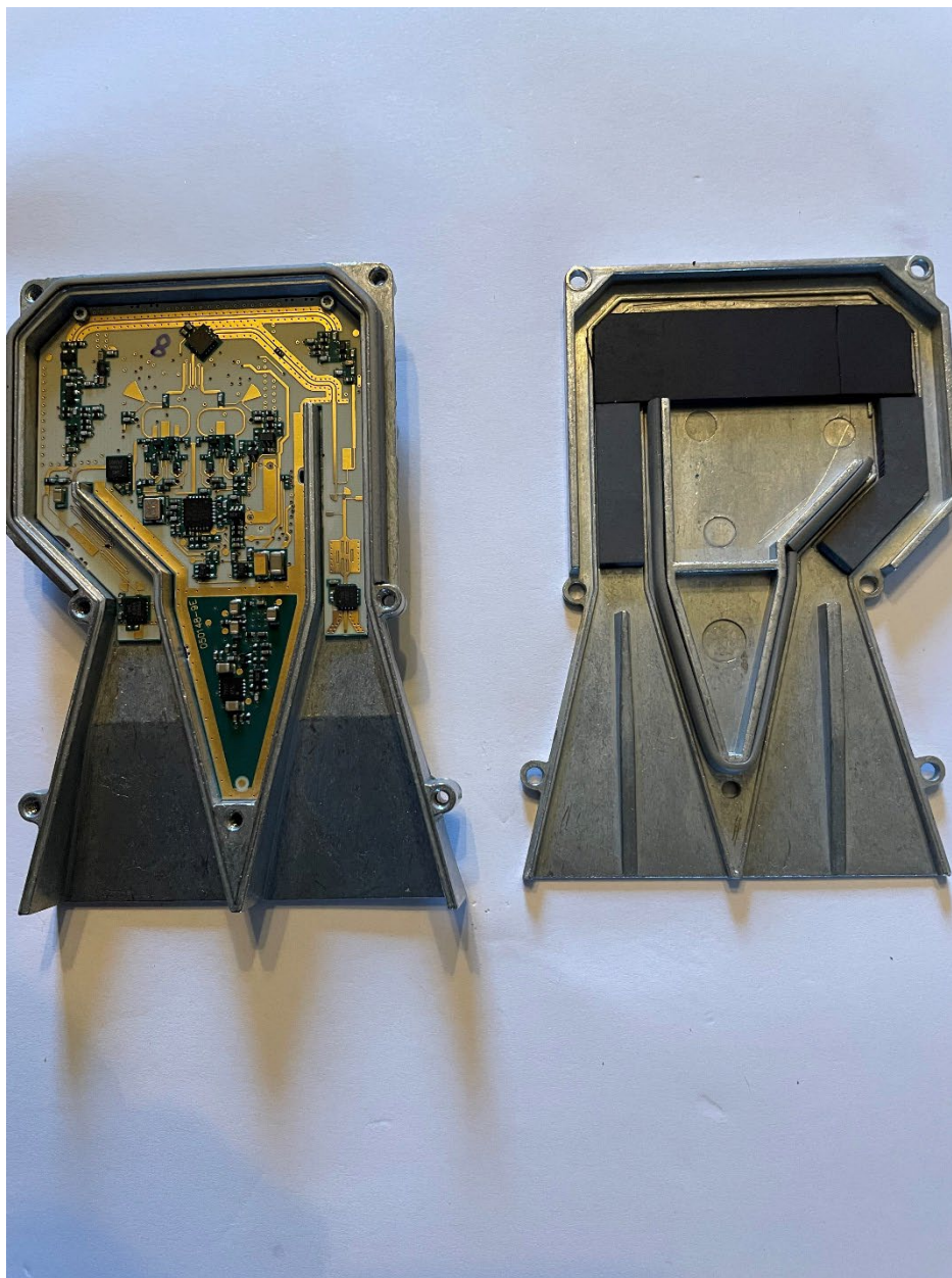
Internal Feedhorn Assembly
