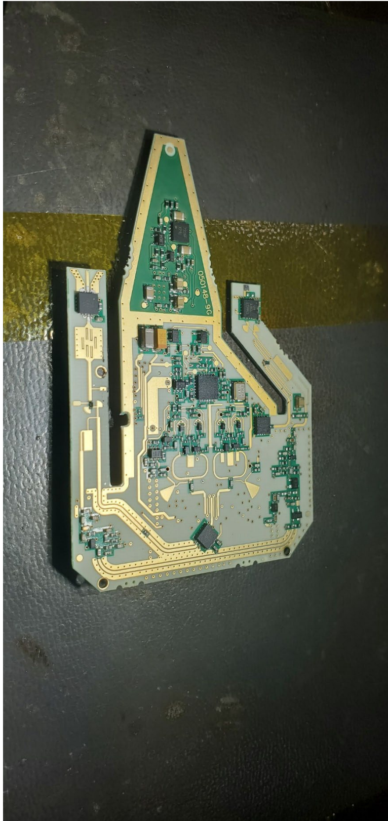
Internal Feedhorn PCB Top View
