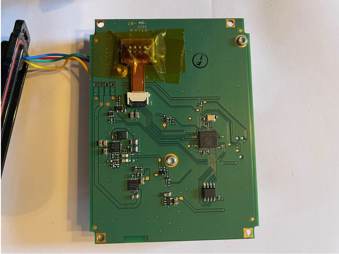
Main PCB Bottom View
