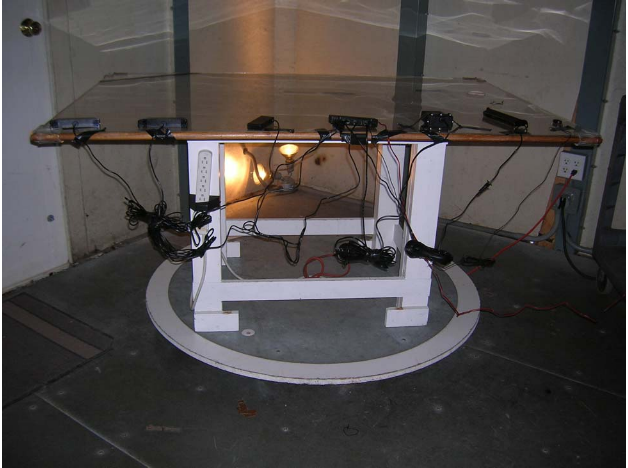
Radiated Emissions
