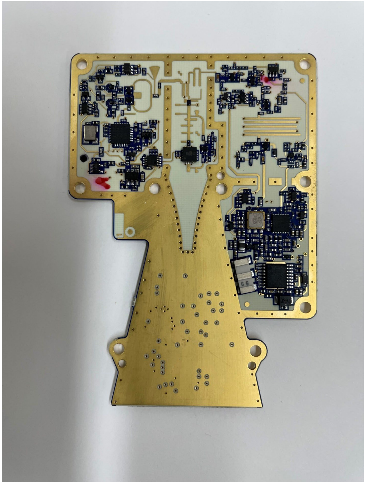
RF Board
