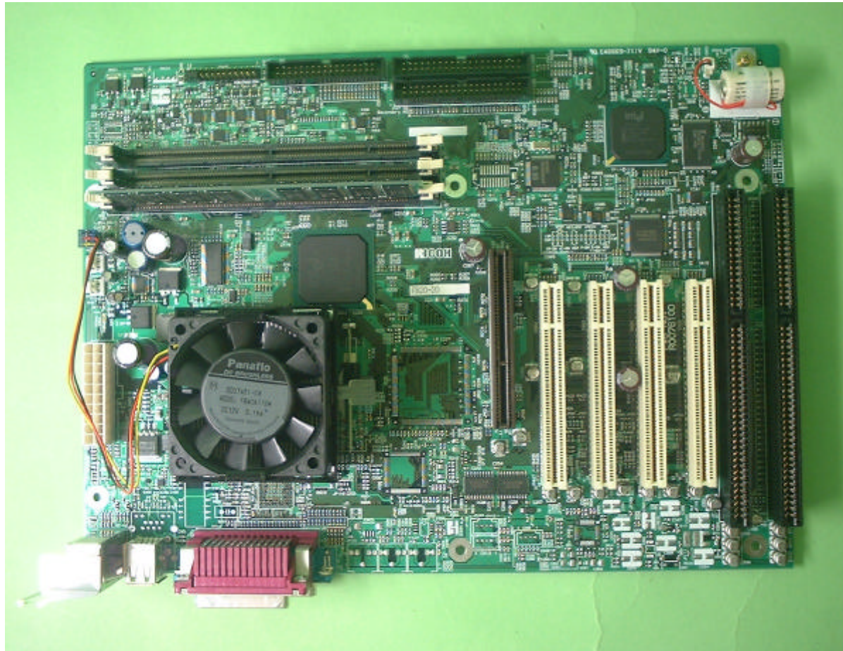
CPU<Top view>
