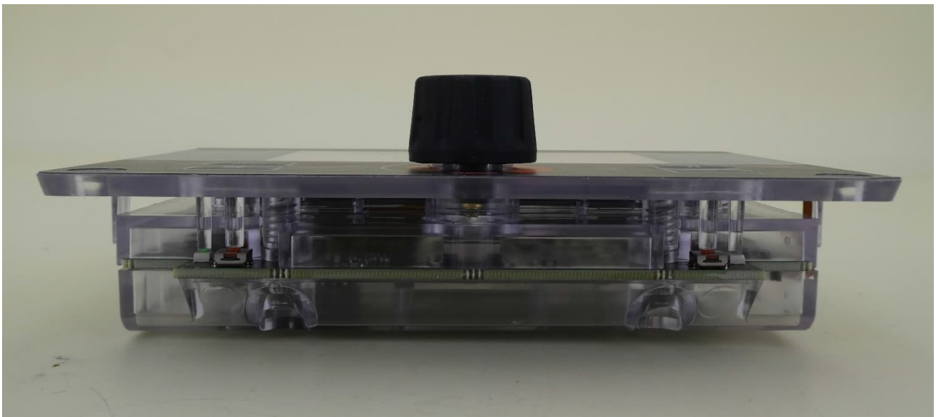
EUT – bottom view
