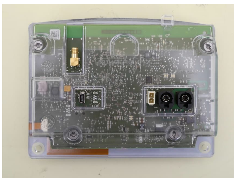
EUT – back view – external antenna removed
