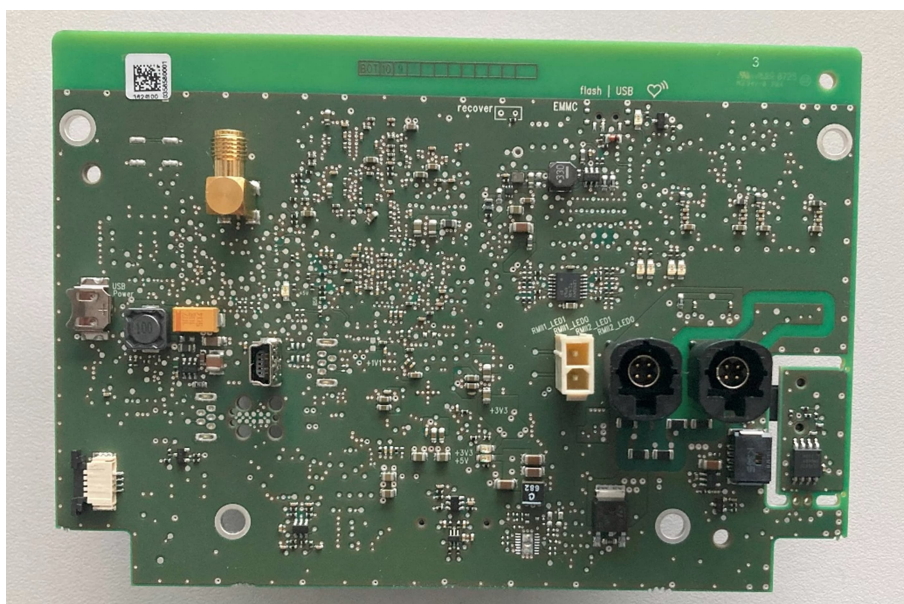
PCB – back view (photograph provided by the applicant)
