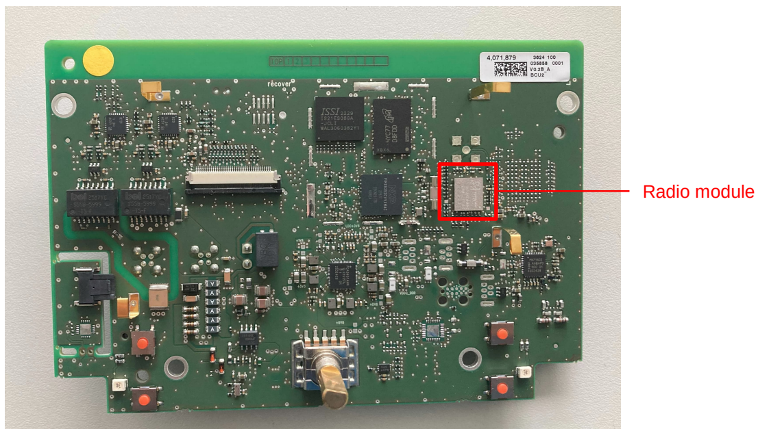
PCB – front view (photograph provided by the applicant)
