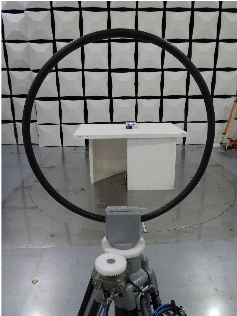
Test setup fully-anechoic chamber M276; Preliminary measurement 9 kHz to 30 MHz
