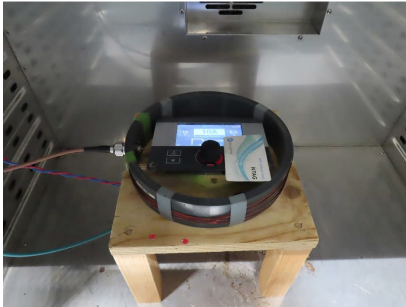
Test setup 99 % bandwidth
