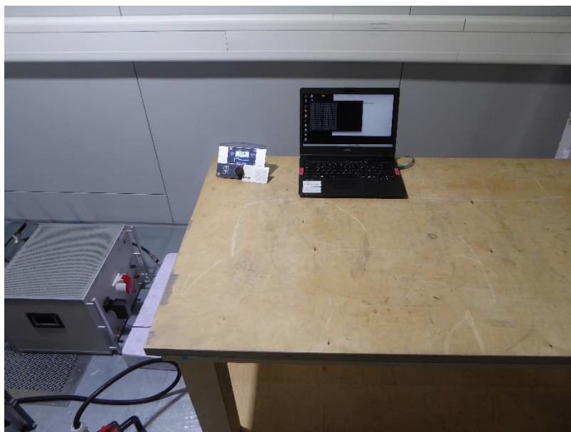
Test setup shielded chamber M155, AC powerline conducted emissions
