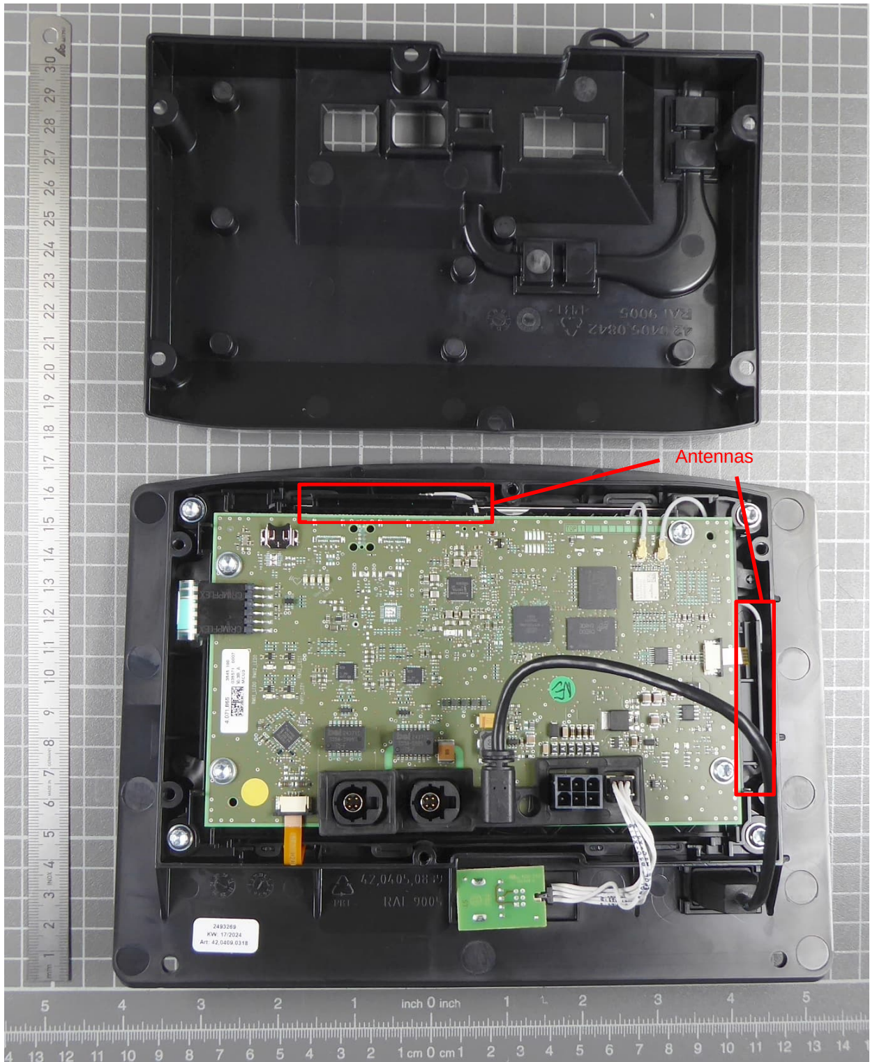
EUT housing opened – view 1
