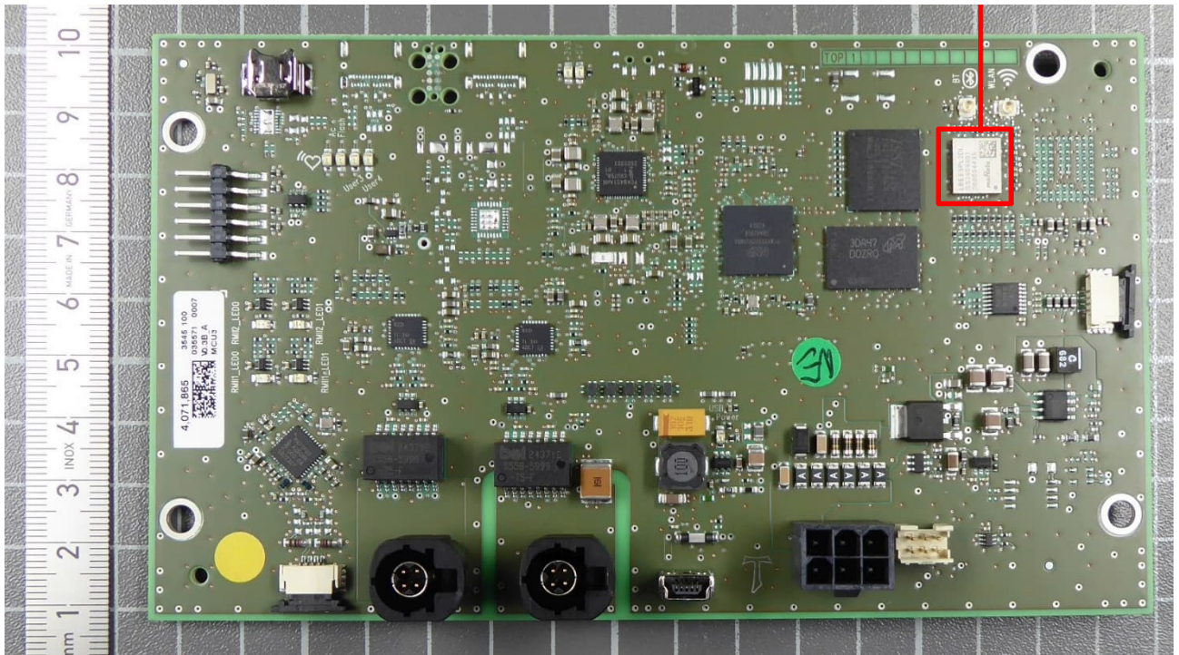
PCB – top view
