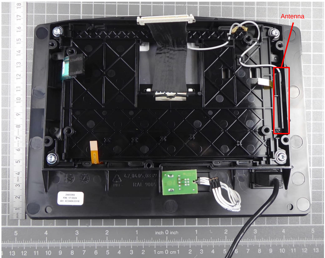
EUT housing opened – view 2
