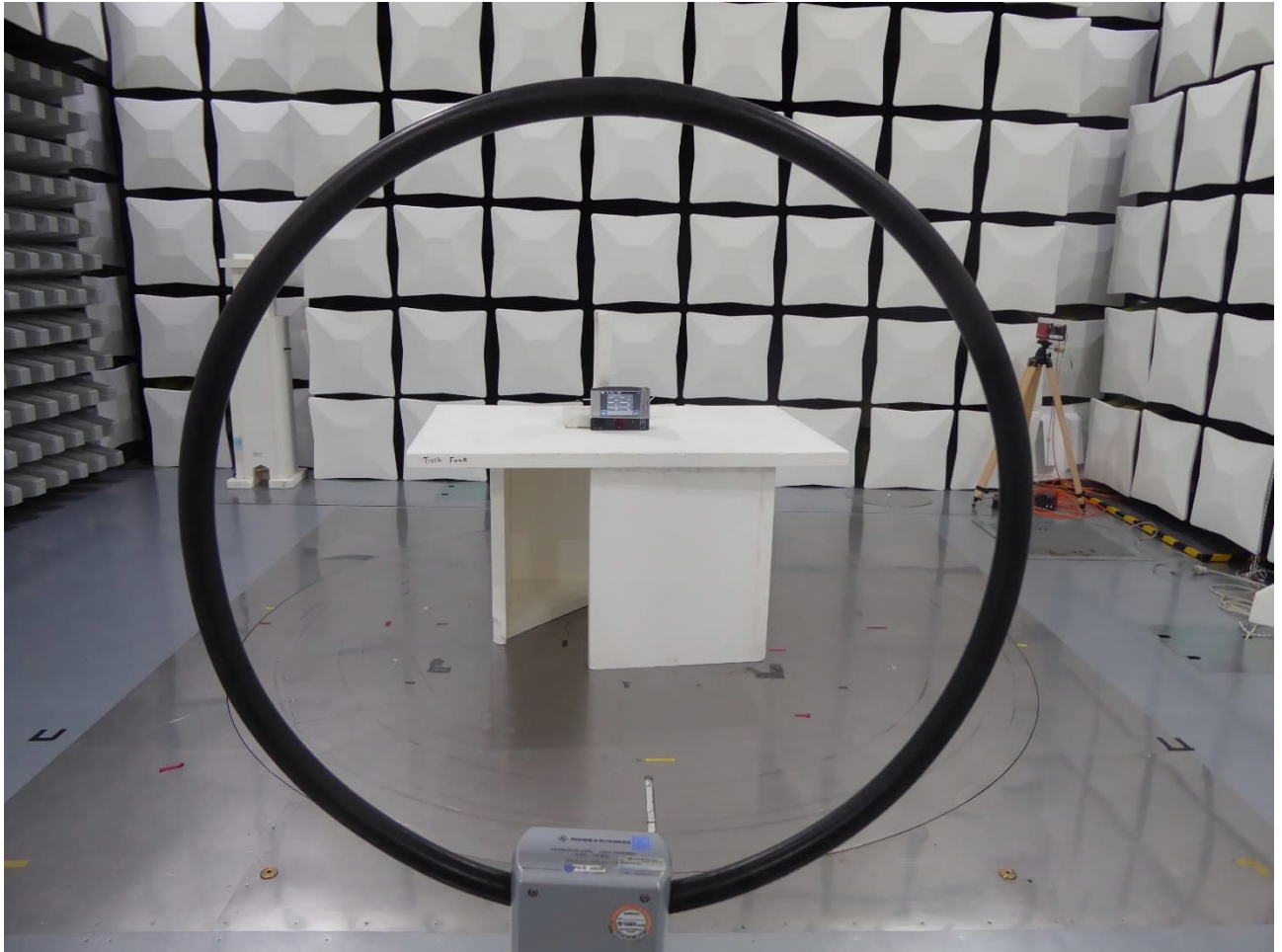
9 kHz – 30 MHz - antenna position 1
