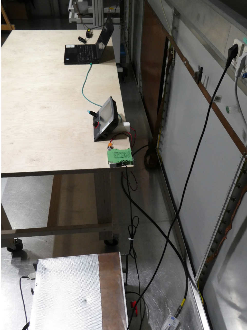
Test setup – AC power line conducted emissions
