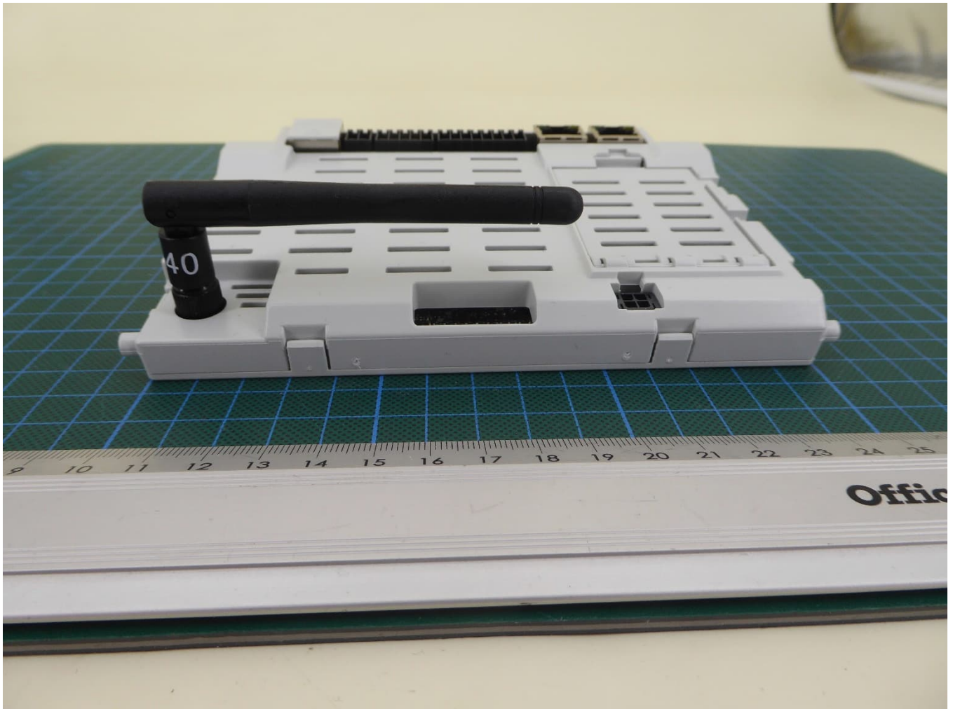
Side view 1
