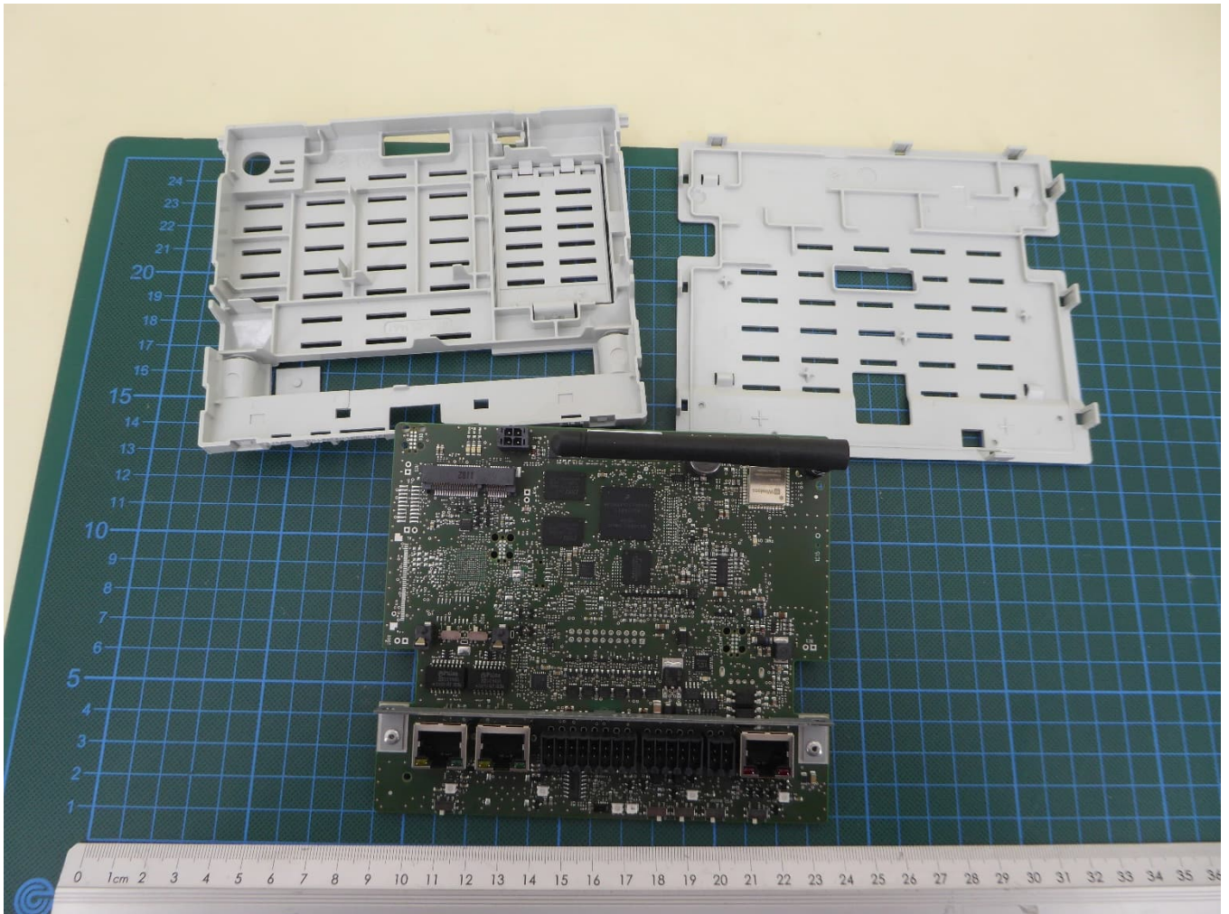
EUT – opened – top view
