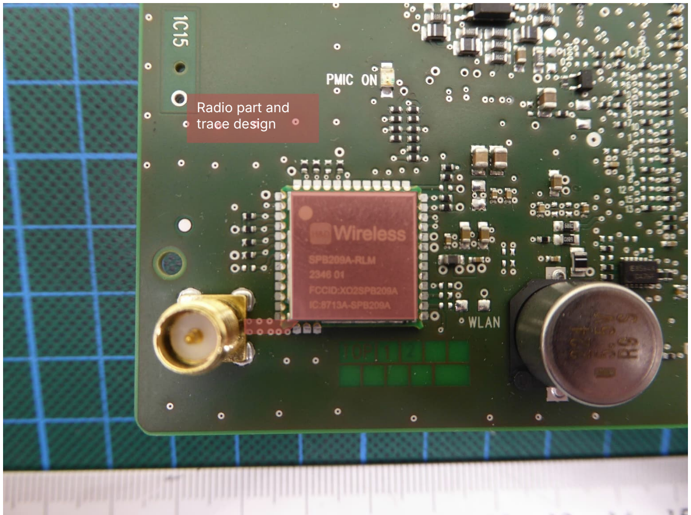
Radio part – detail view
