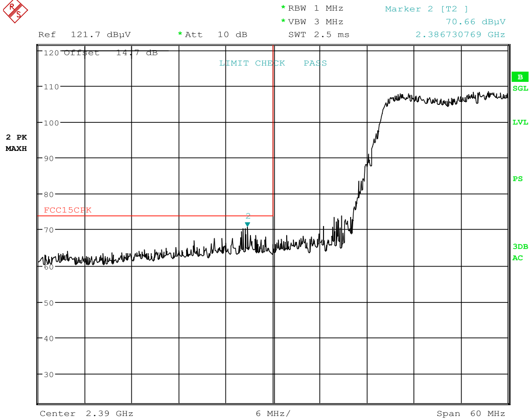
Plot 7-16. Radiated Restricted Lower Band Edge Measurement (Peak)
