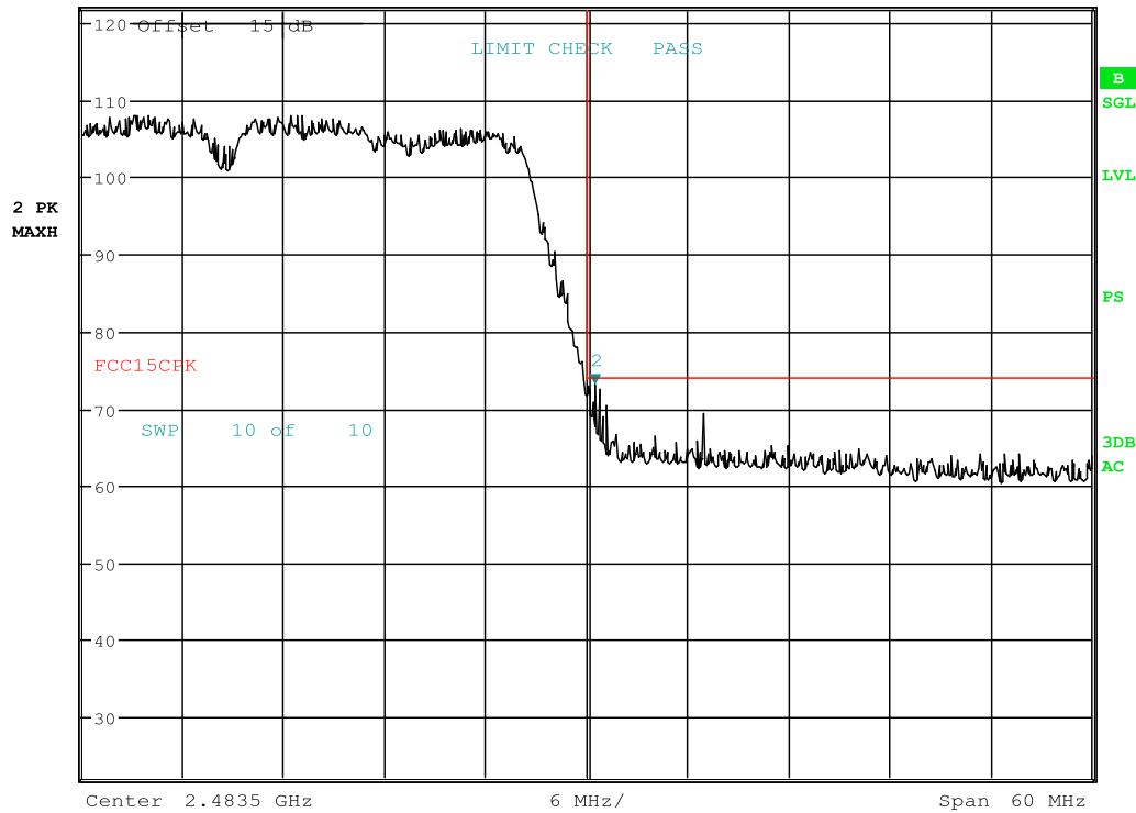
Plot 7-20. Radiated Restricted Upper Band Edge Measurement (Peak)
