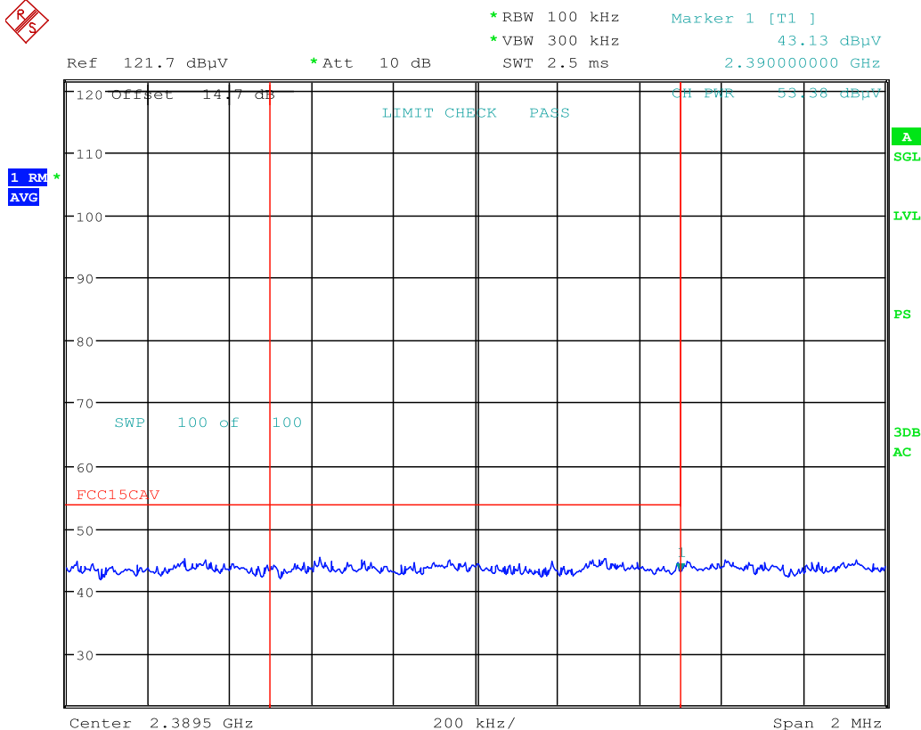
Plot 7-15. Radiated Restricted Lower Band Edge Measurement (Average)
