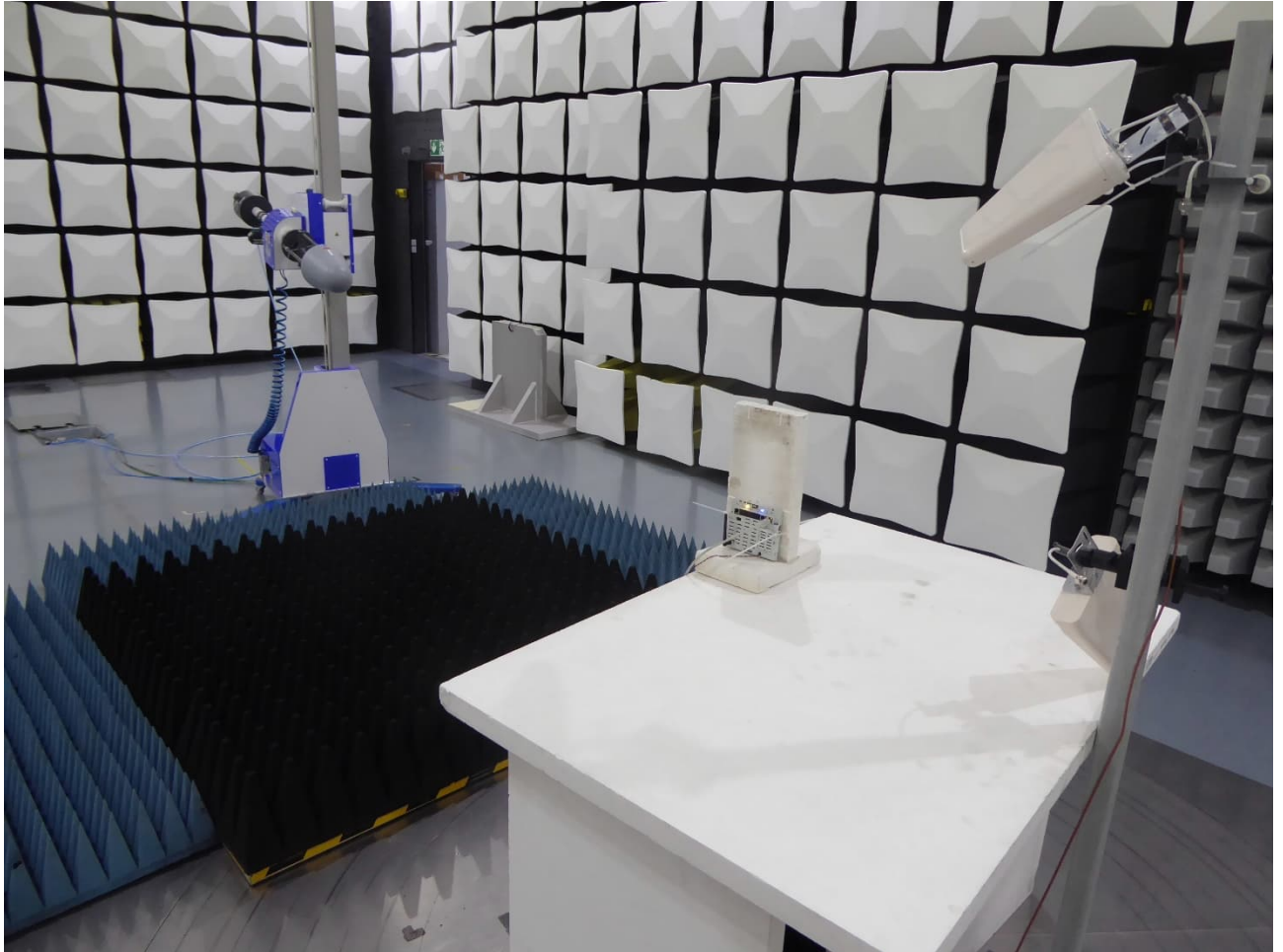
1 GHz – 13 GHz
