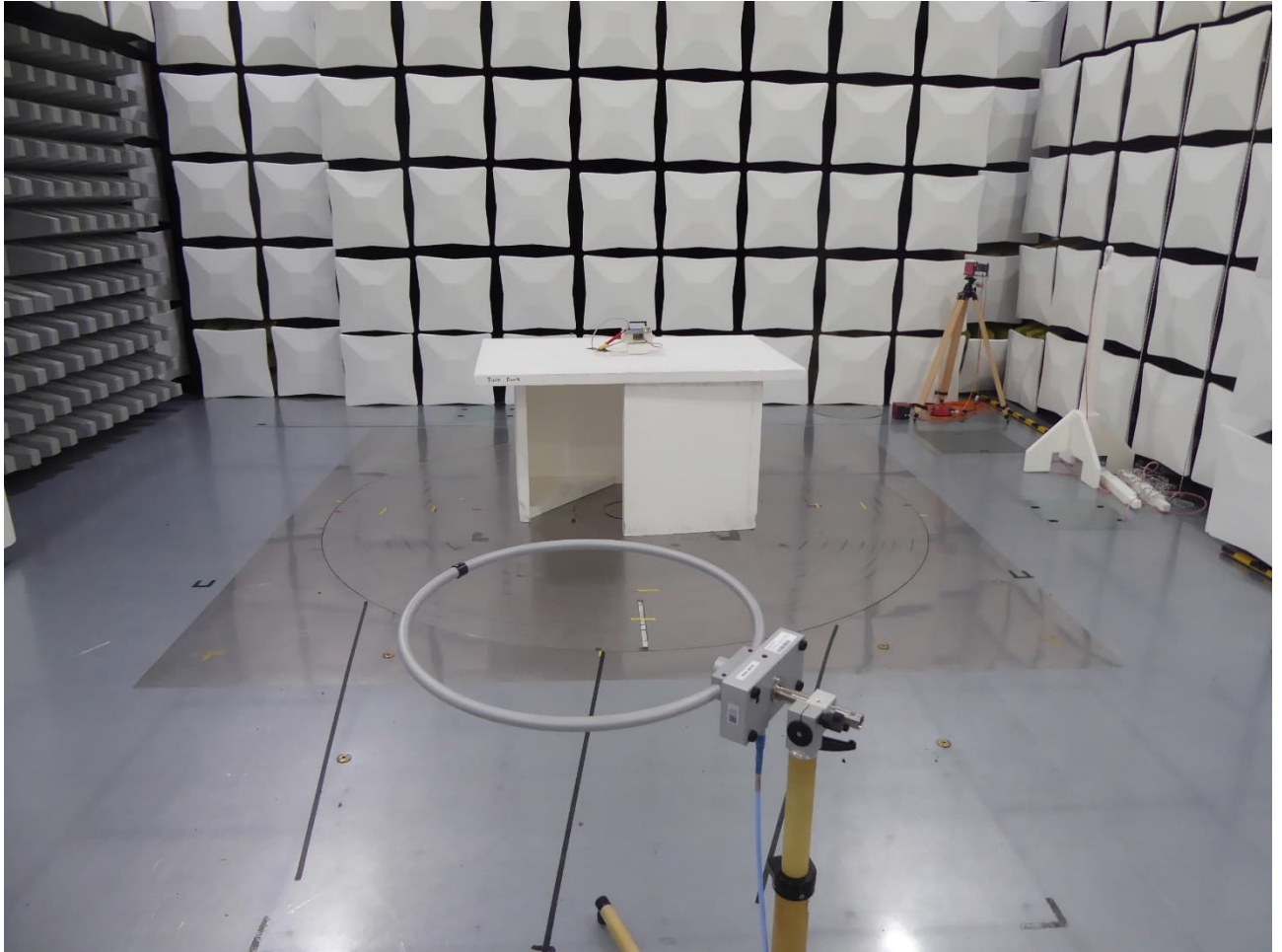
9 kHz – 30 MHz – Antenna Position 3
