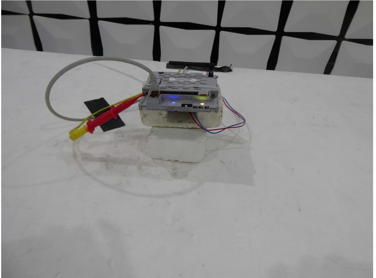
EUT Position 3 below 1GHz
