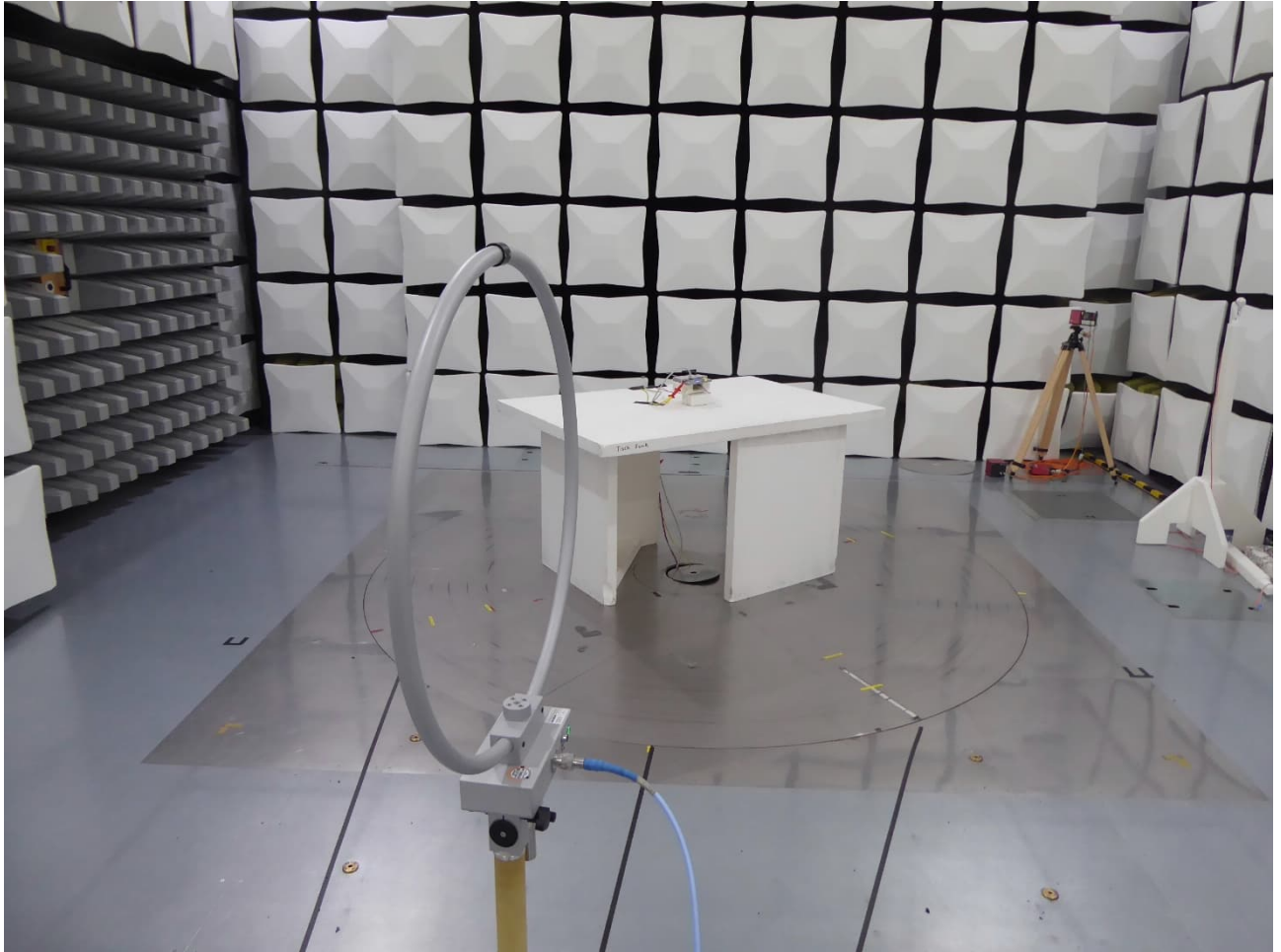
9 kHz – 30 MHz – Antenna Position 2
