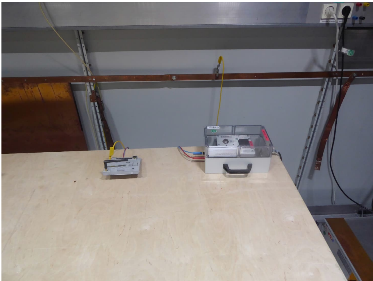
AC powerline conducted measurement
