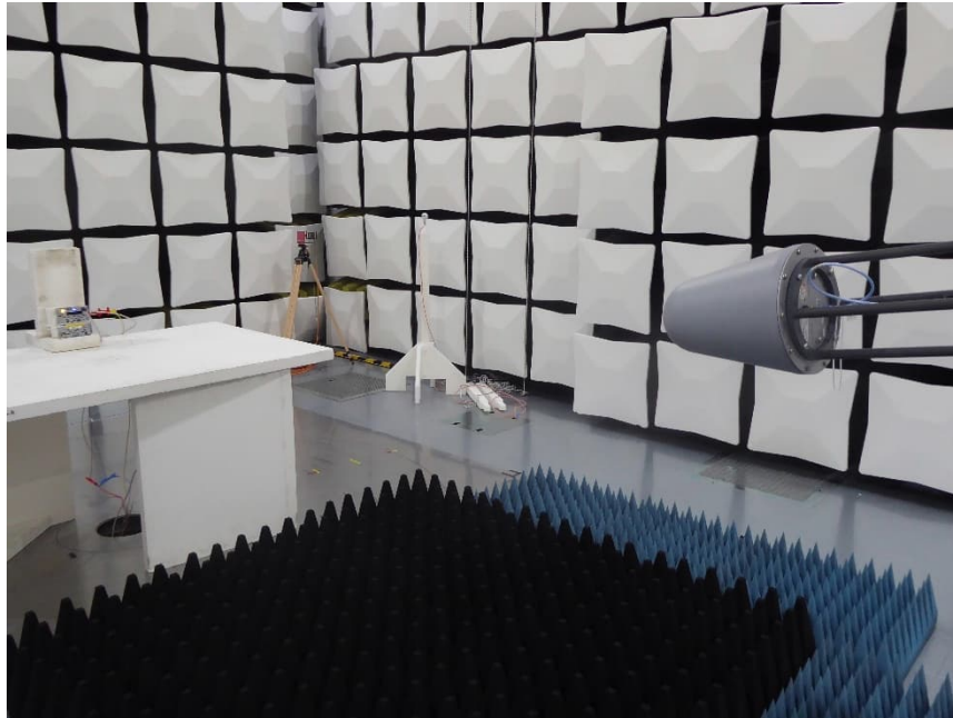
Test setup semi anechoic chamber with ground absorber M276 Preliminary and final measurement 1 GHz - 13 GHz
