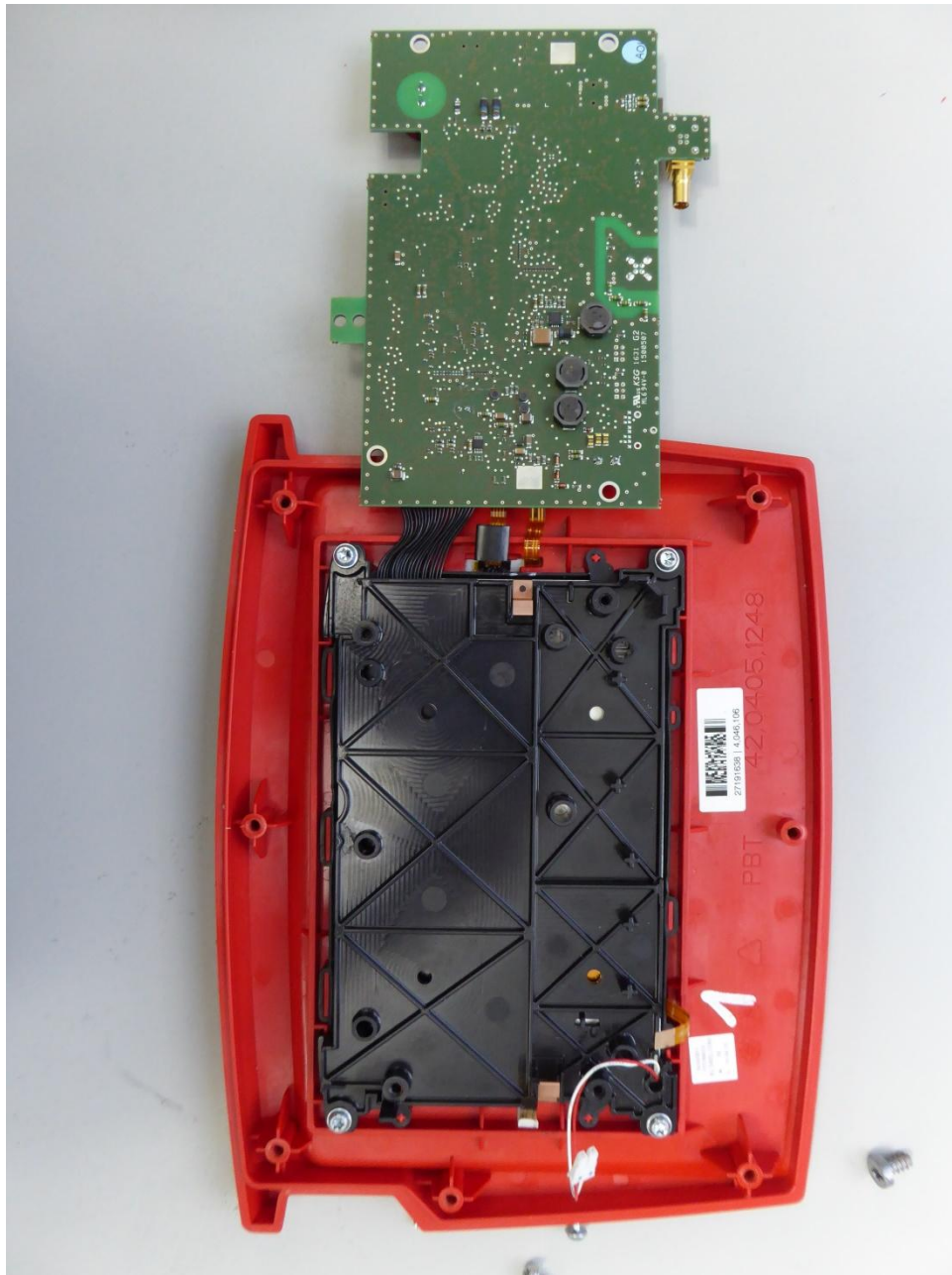
161548_12.JPG: RC Panel Pro, internal view 3
