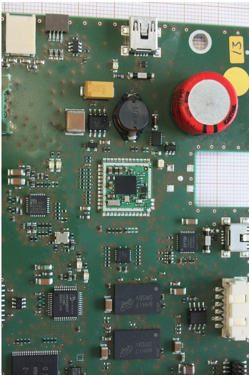
161548_17.JPG: RC Panel Pro, detail view to radio module (shielding removed)
