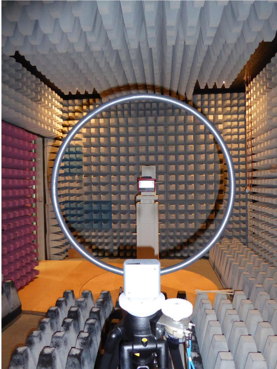
161548_1.JPG: Test setup fully anechoic chamber
