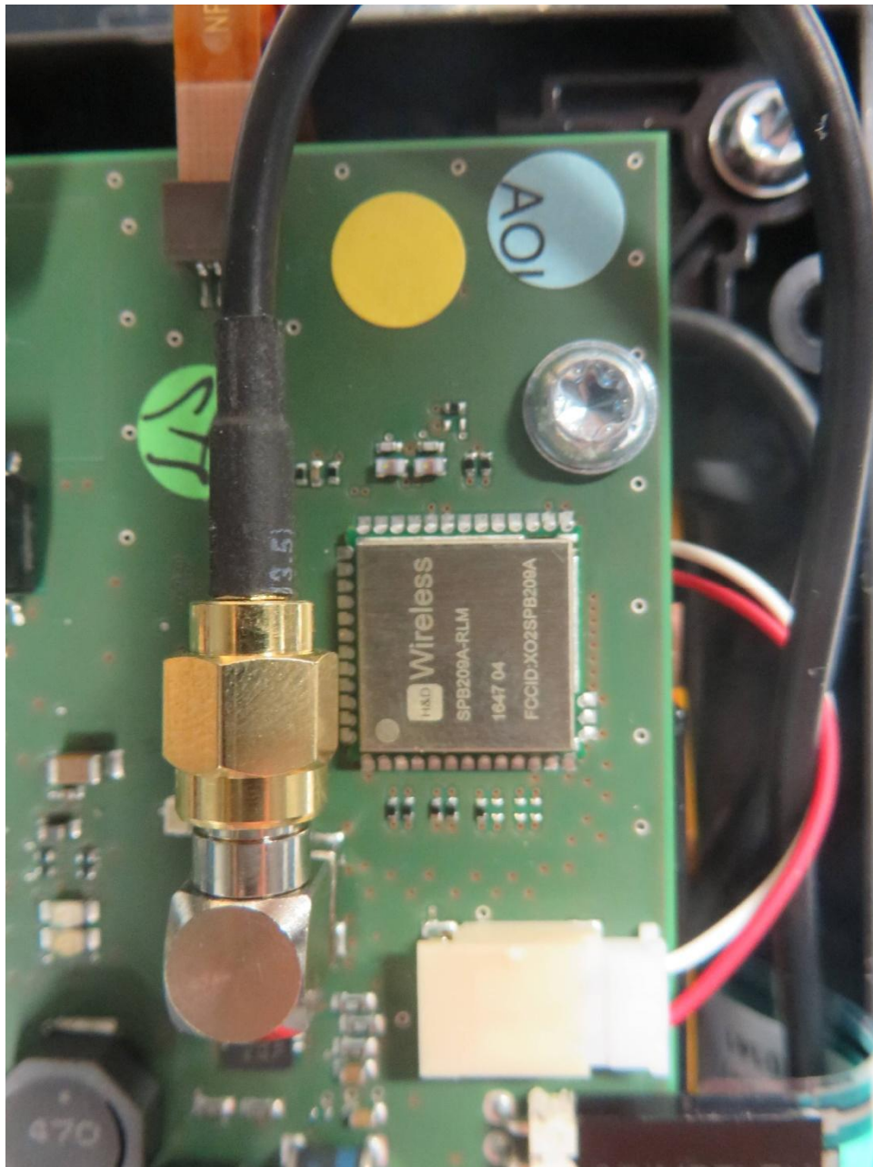
EUT Radio module – detail view
