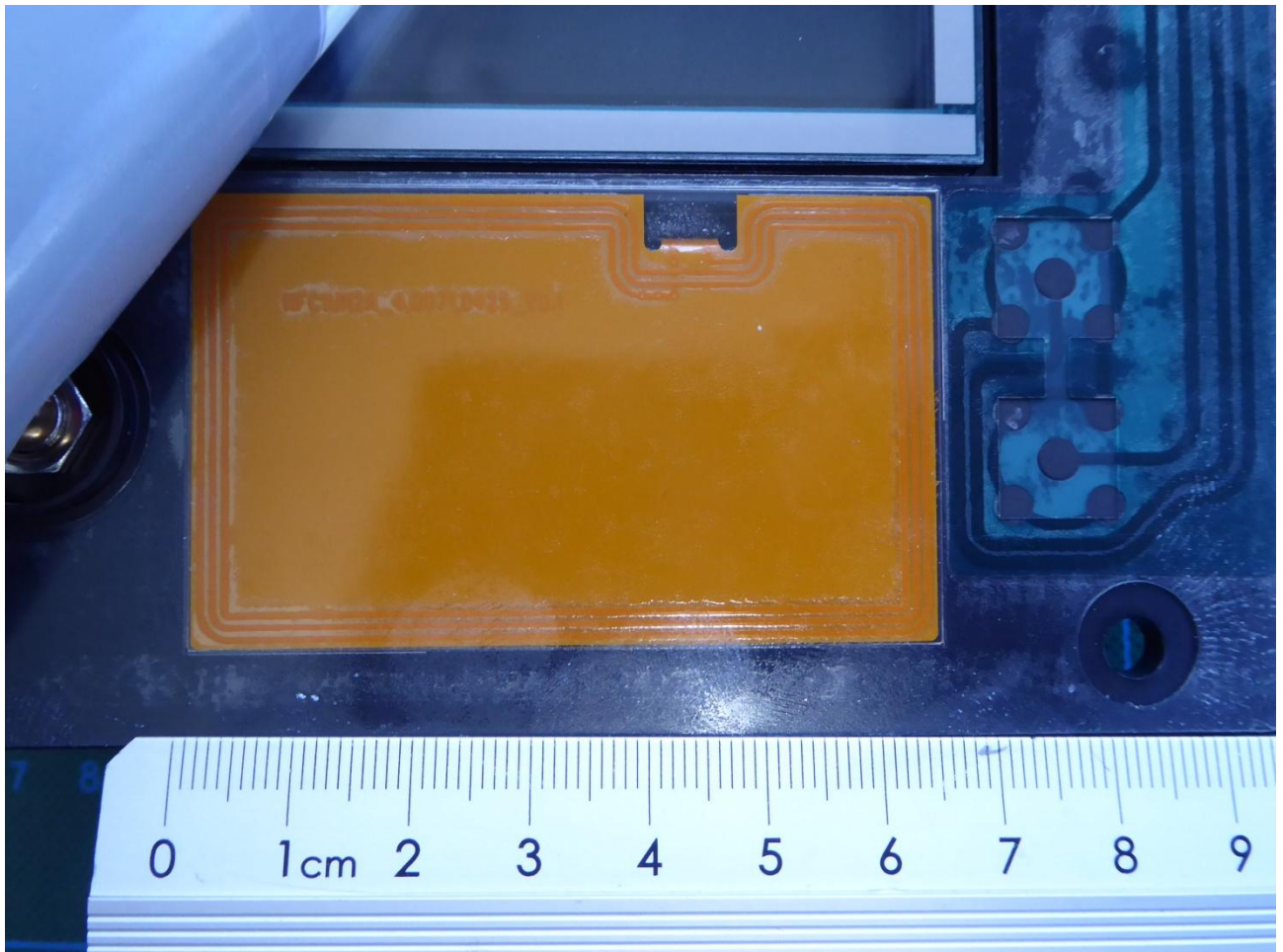
NFC antenna detail view
