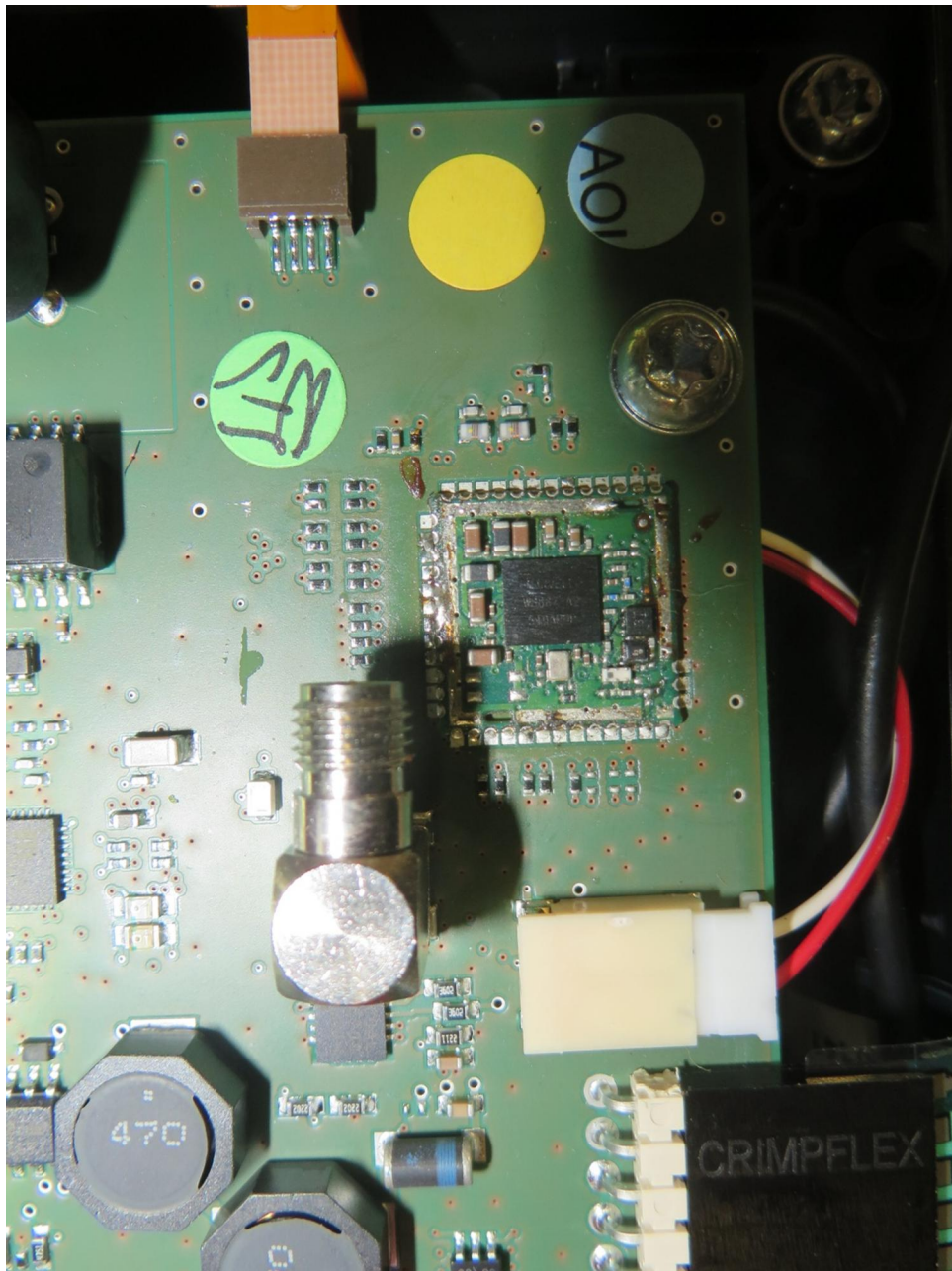
EUT Radio module – detail view w/o screening
