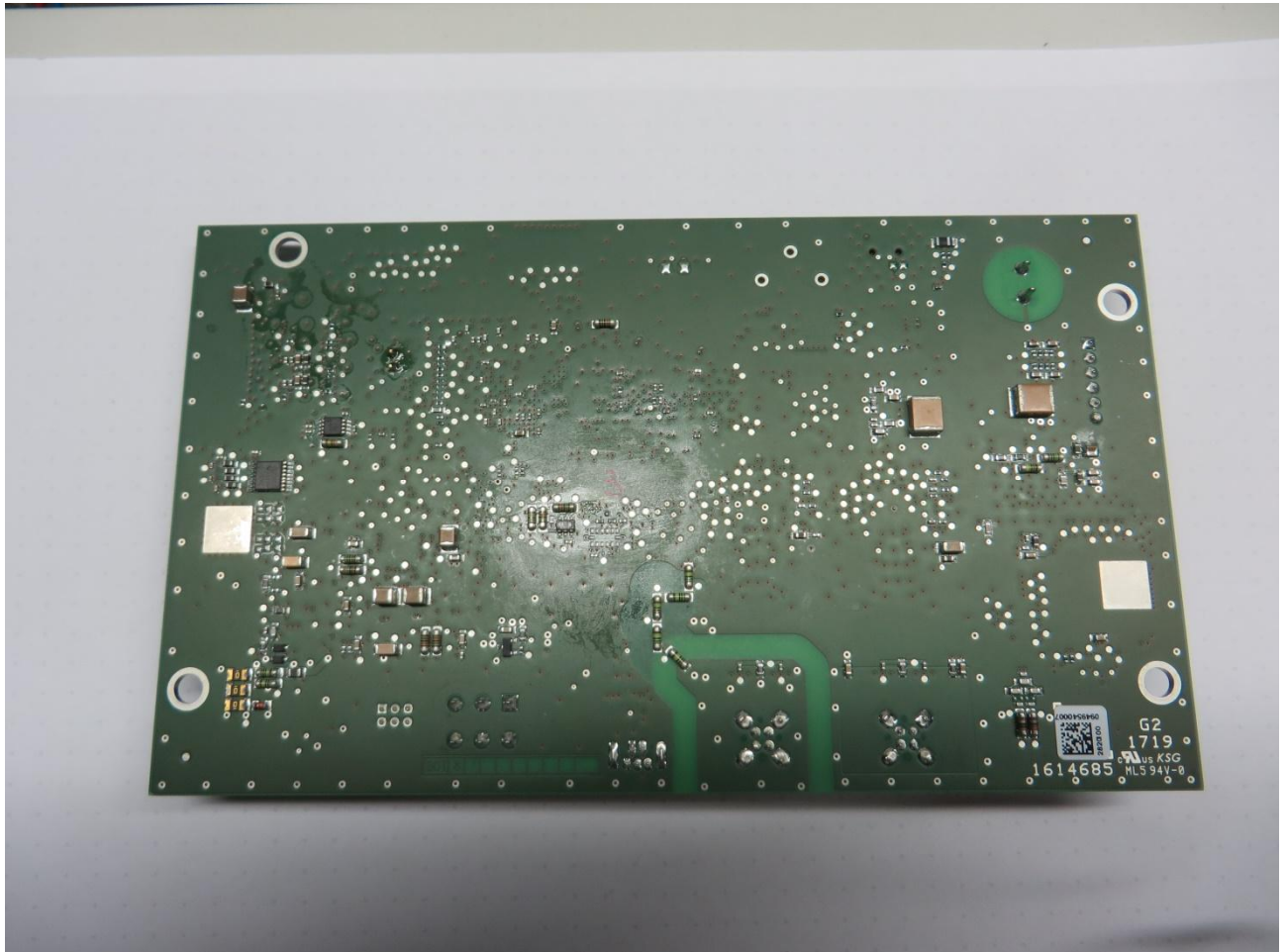
EUT PCB – bottom view
