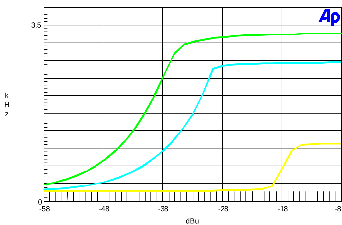
Modulation Limiting Plot: 2.5KHz, 1KHz, 300Hz
