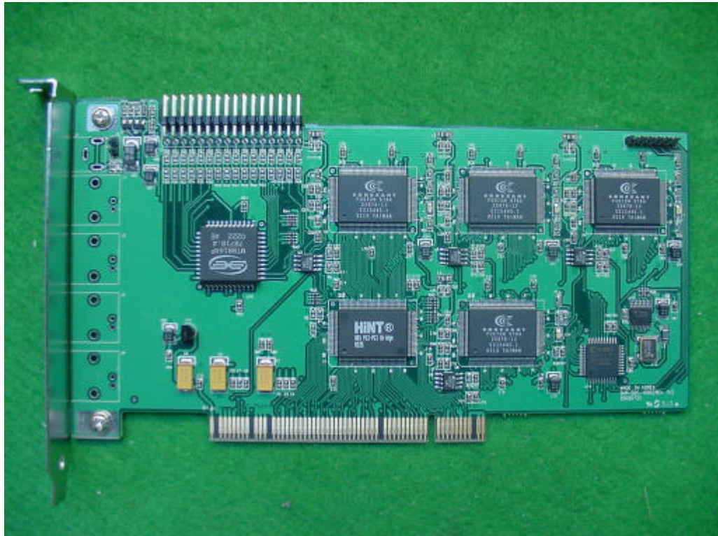
CAPTURE BOARD (FRONT)
