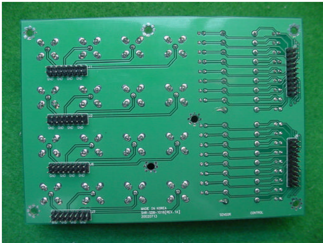
BNCBOARD(BNC16)(FRONT)
