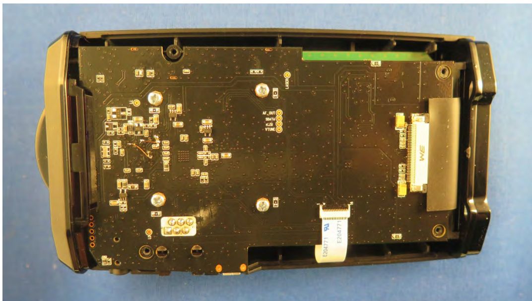
MAIN PCB IN CASE
