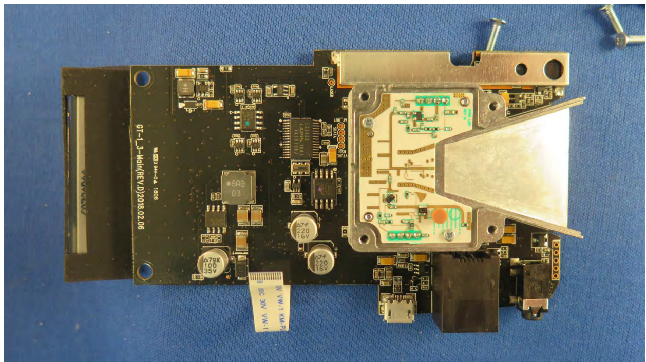
MAIN PCB – TOP VIEW – UPPER HORN REMOVED
