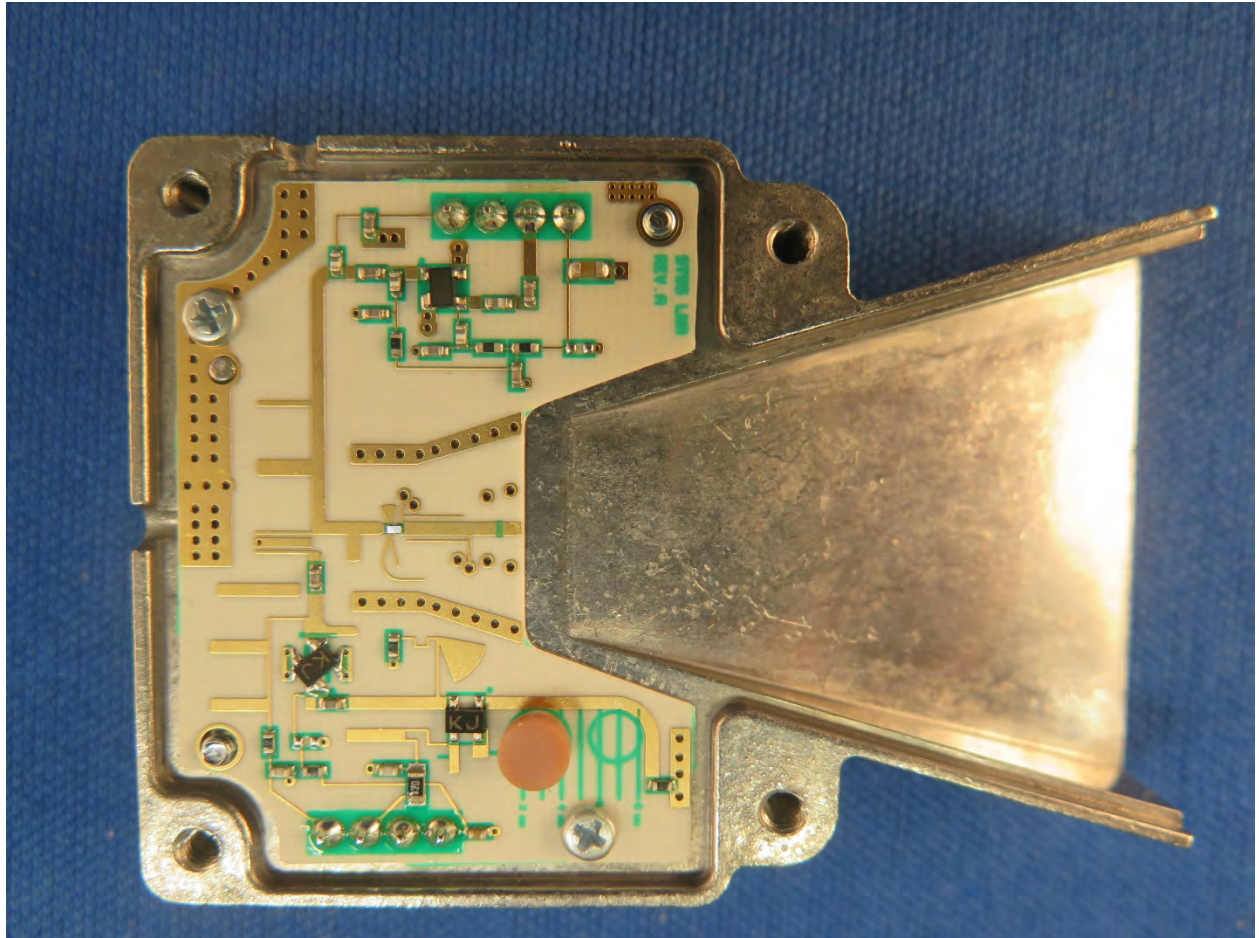
HORN LOWER WITH LNA PCB
