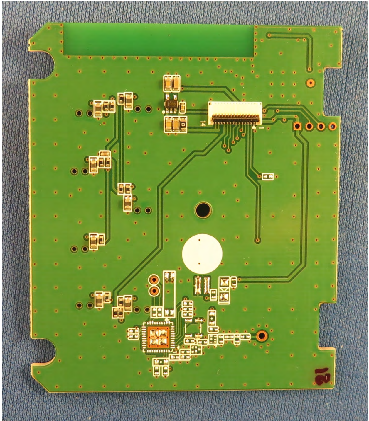
SUB PCB – BOTTOM VIEW
