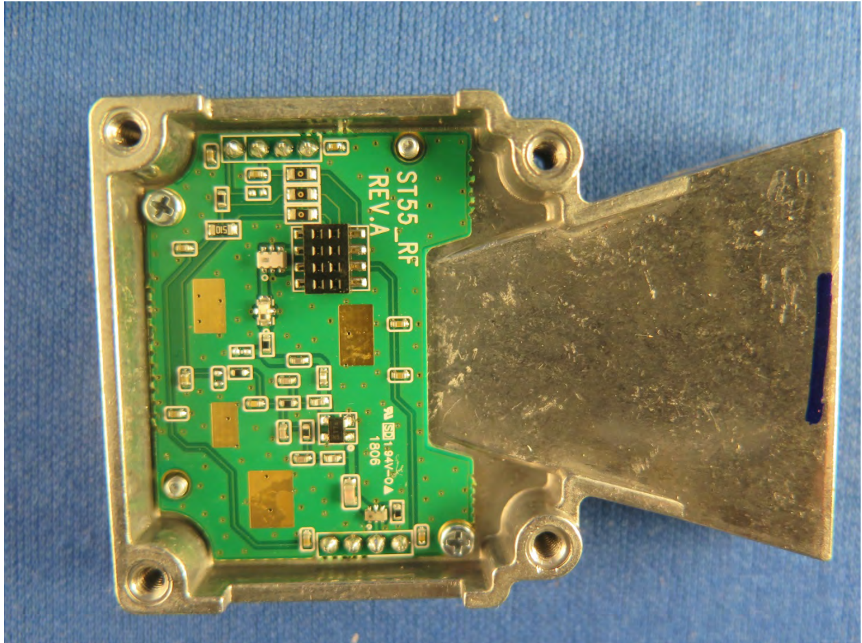
HORN LOWER WITH RF PCB
