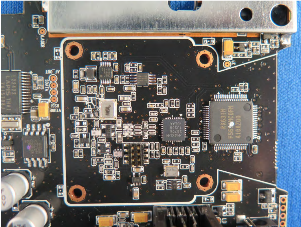
TOP VIEW MAIN PCB HORN REMOVED – CLOSE UP
