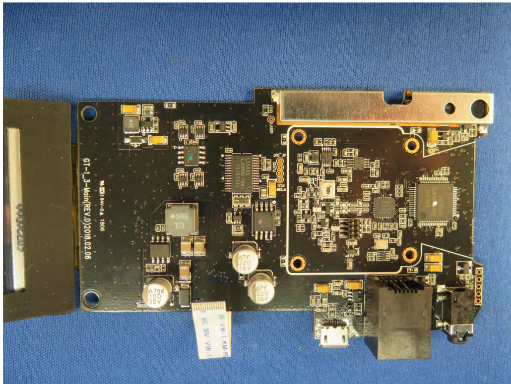
MAIN PCB HORN REMOVED – TOP VIEW
