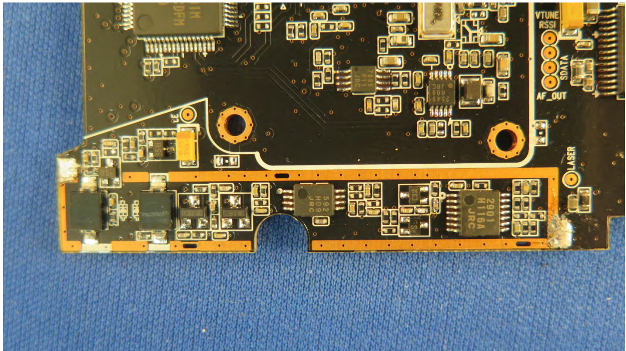
MAIN PCB – TOP VIEW LASER SHIELD REMOVED
