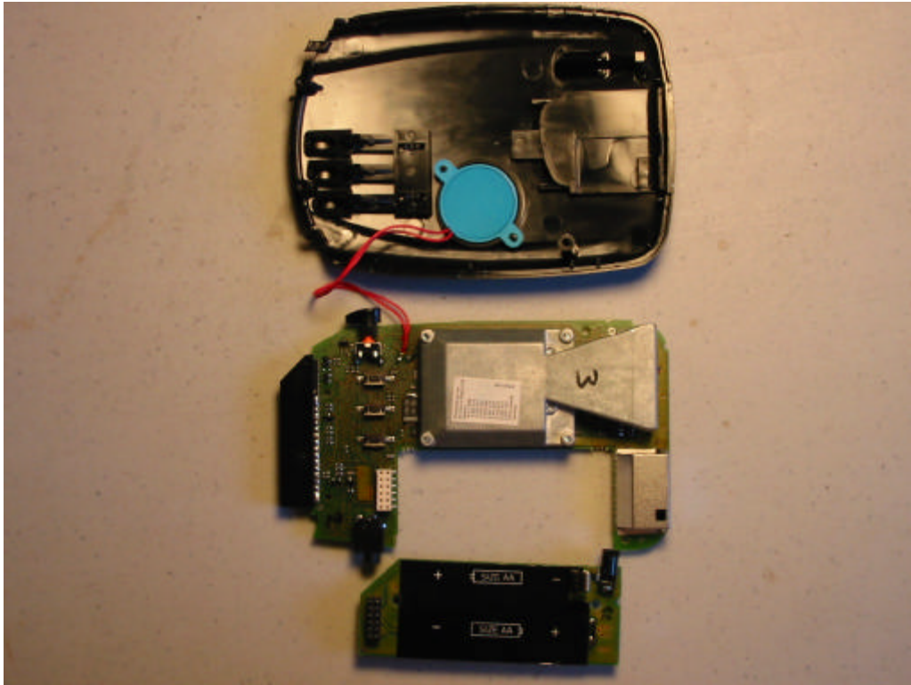
Model: Express Cordless 946 FCC ID: QL4G5S6A
