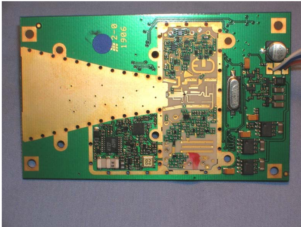
Radar Detector PCB with Waveguide removed
