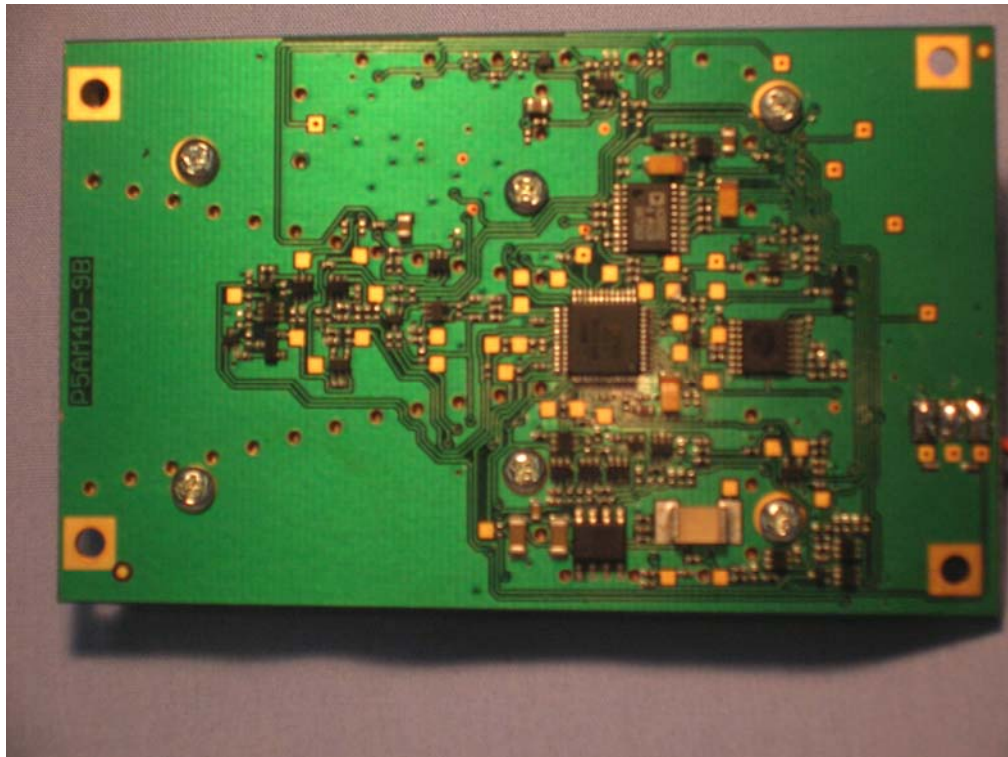
Radar Detector PCB Bottom View
