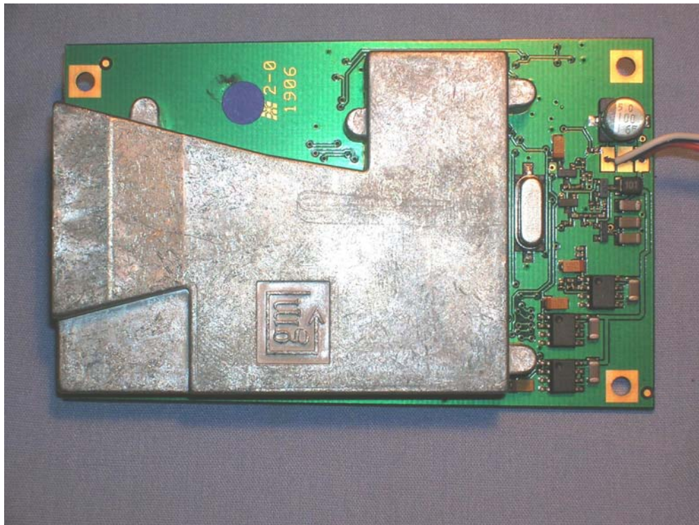
Radar Detector PCB Top View
