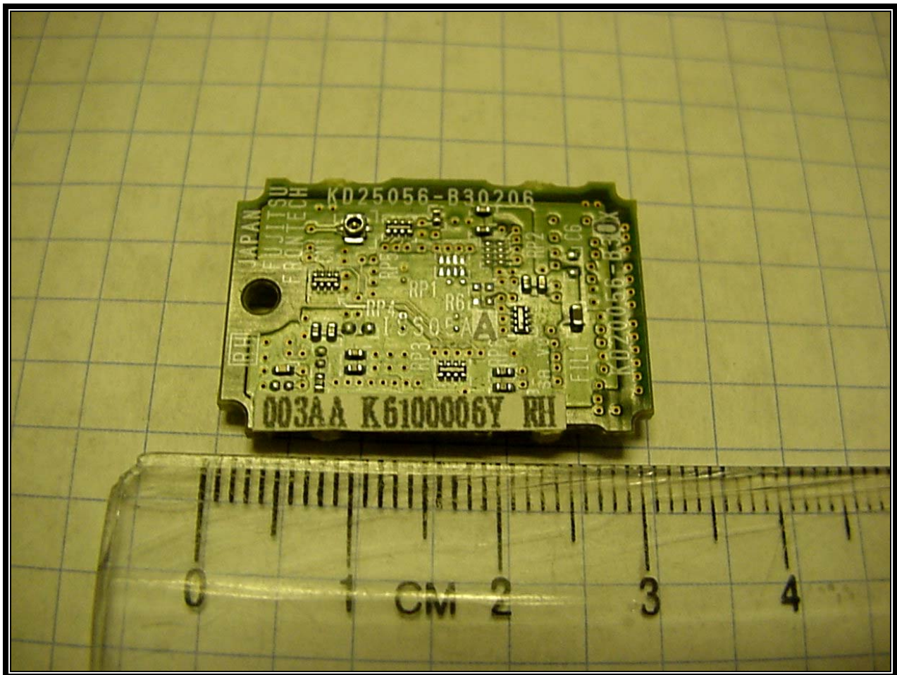
Photograph 17: Back of WLAN Radio PCB
