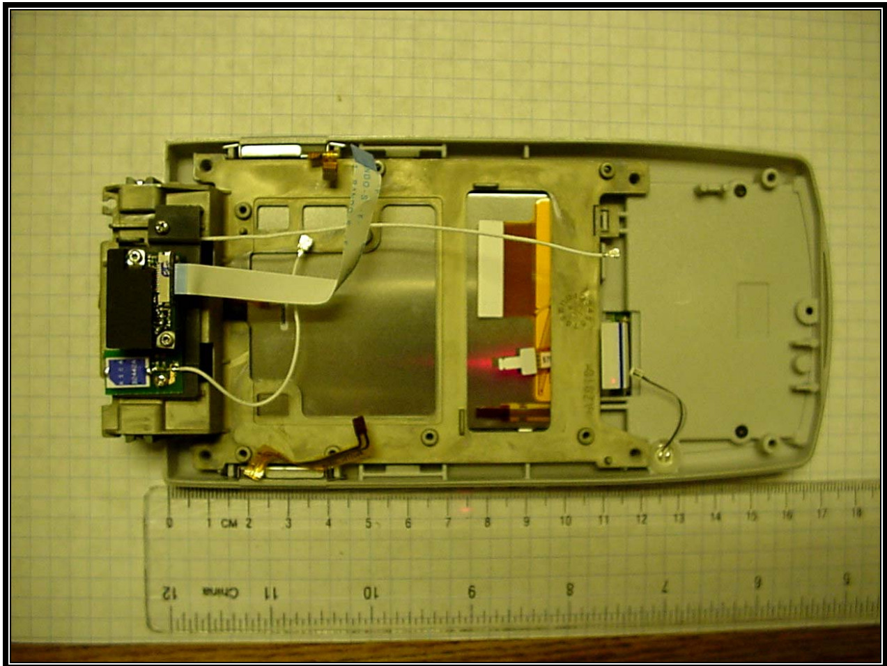
Photograph 20: Front Case with PCB Removed
