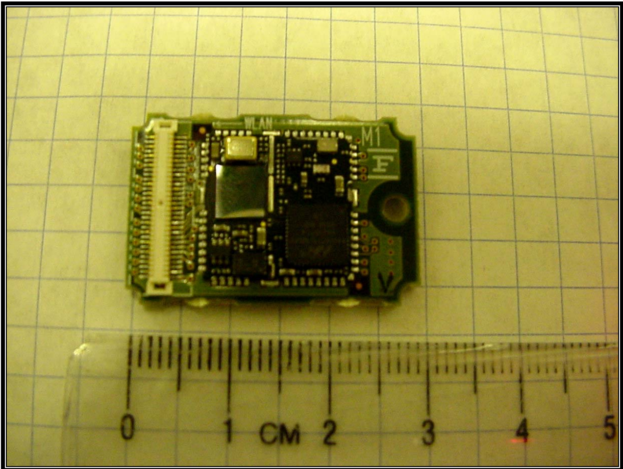
Photograph 16: Front of WLAN Radio PCB with Shield Removed
