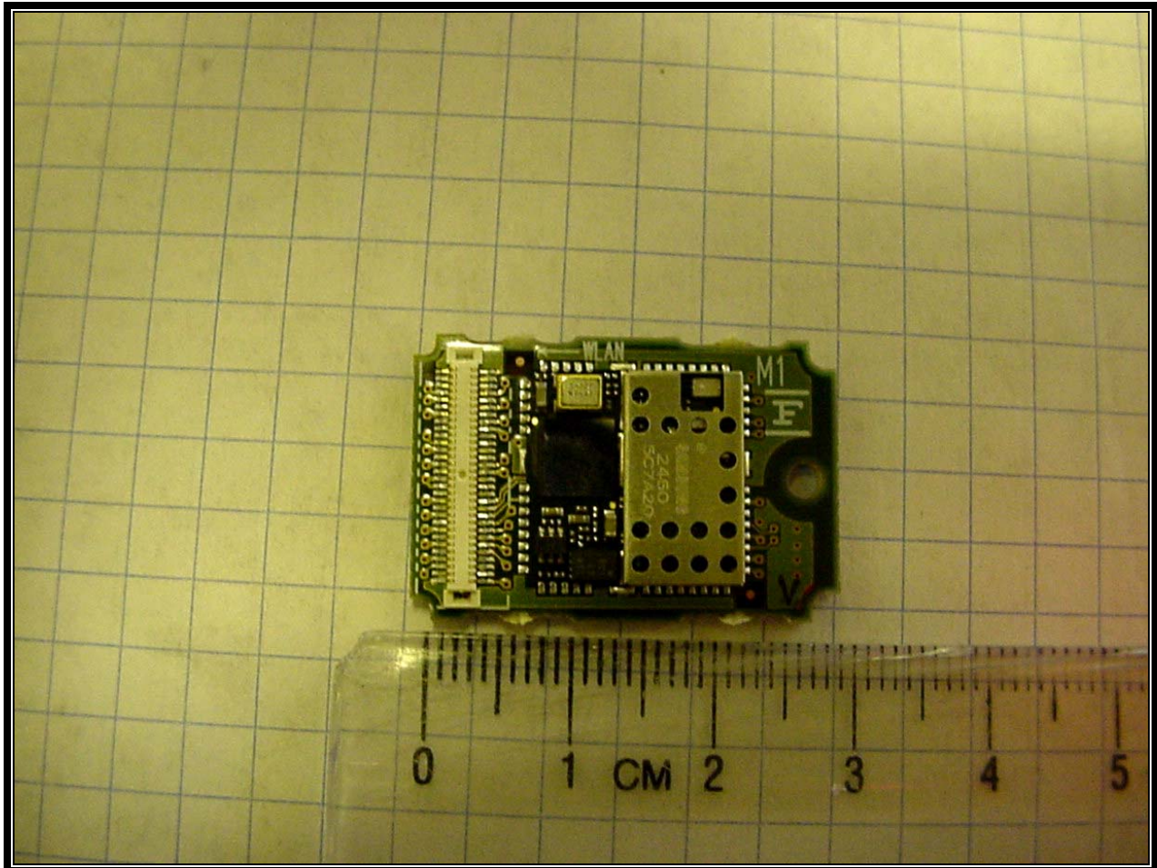
Photograph 15: Front of WLAN Radio PCB with Shield
