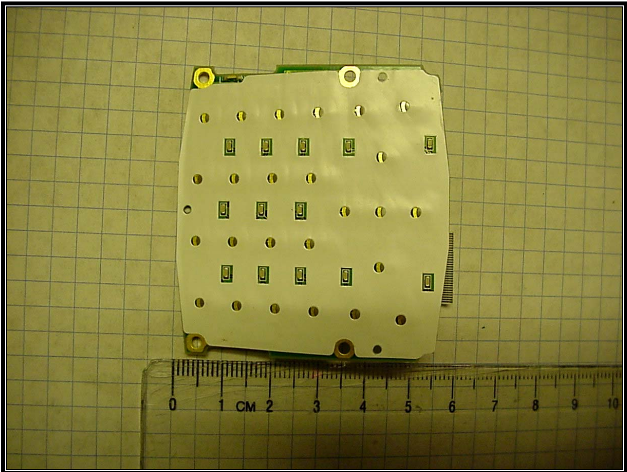
Photograph 22: Front of Keypad PCB
