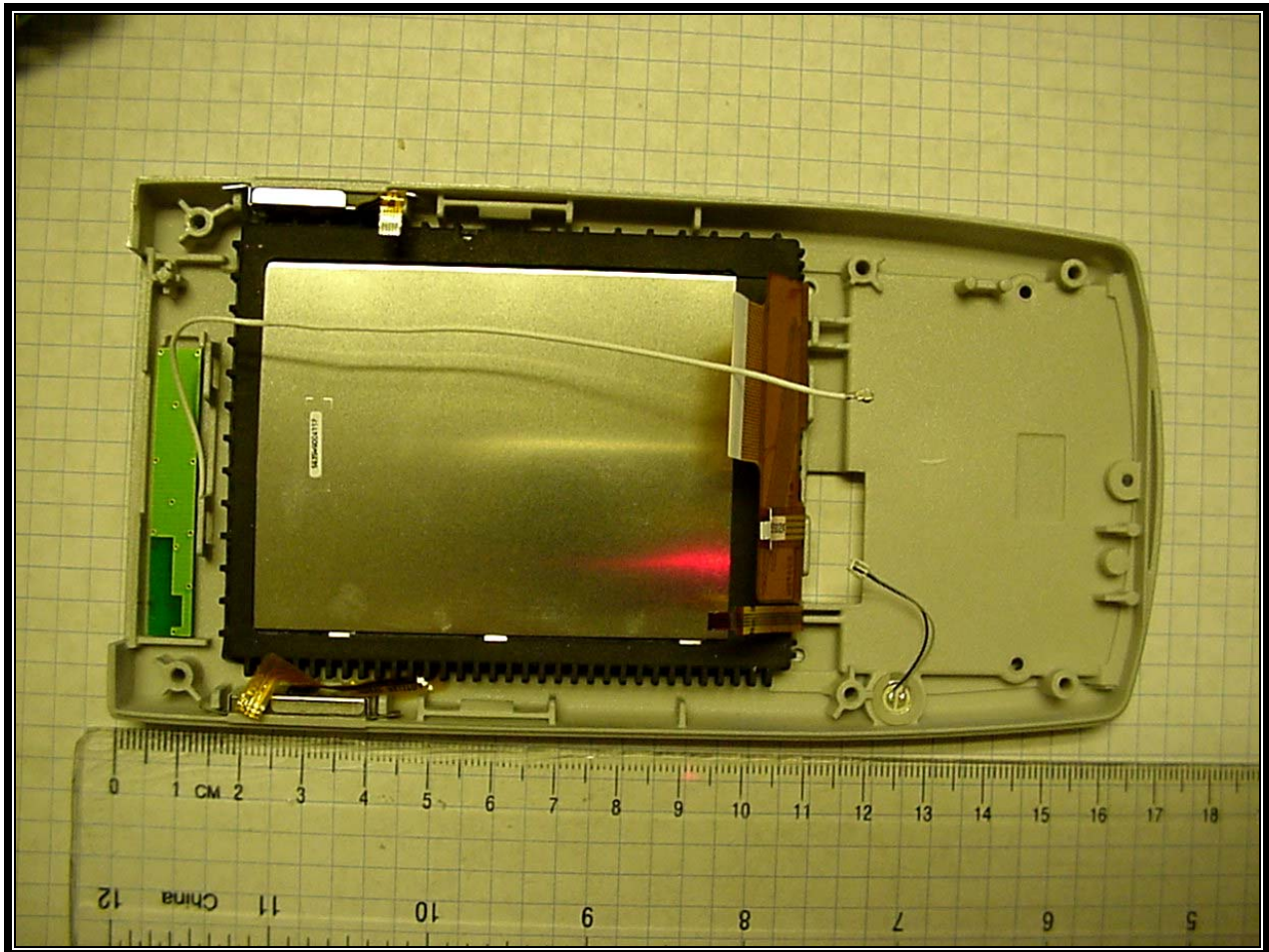
Photograph 21: LCD in Front Case
