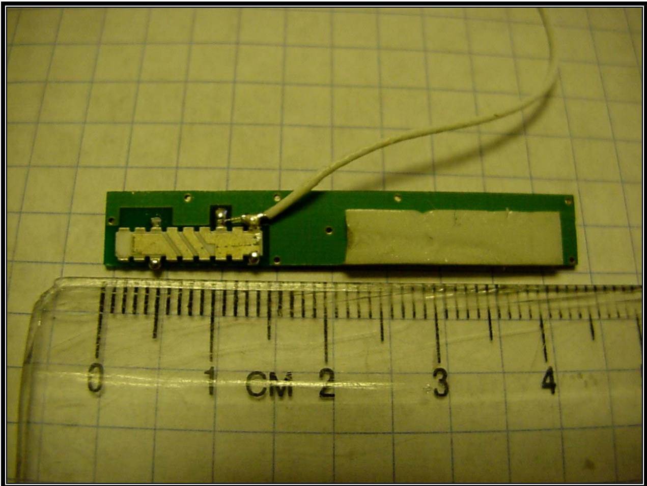
Photograph 18: WLAN Antenna - Front Side
