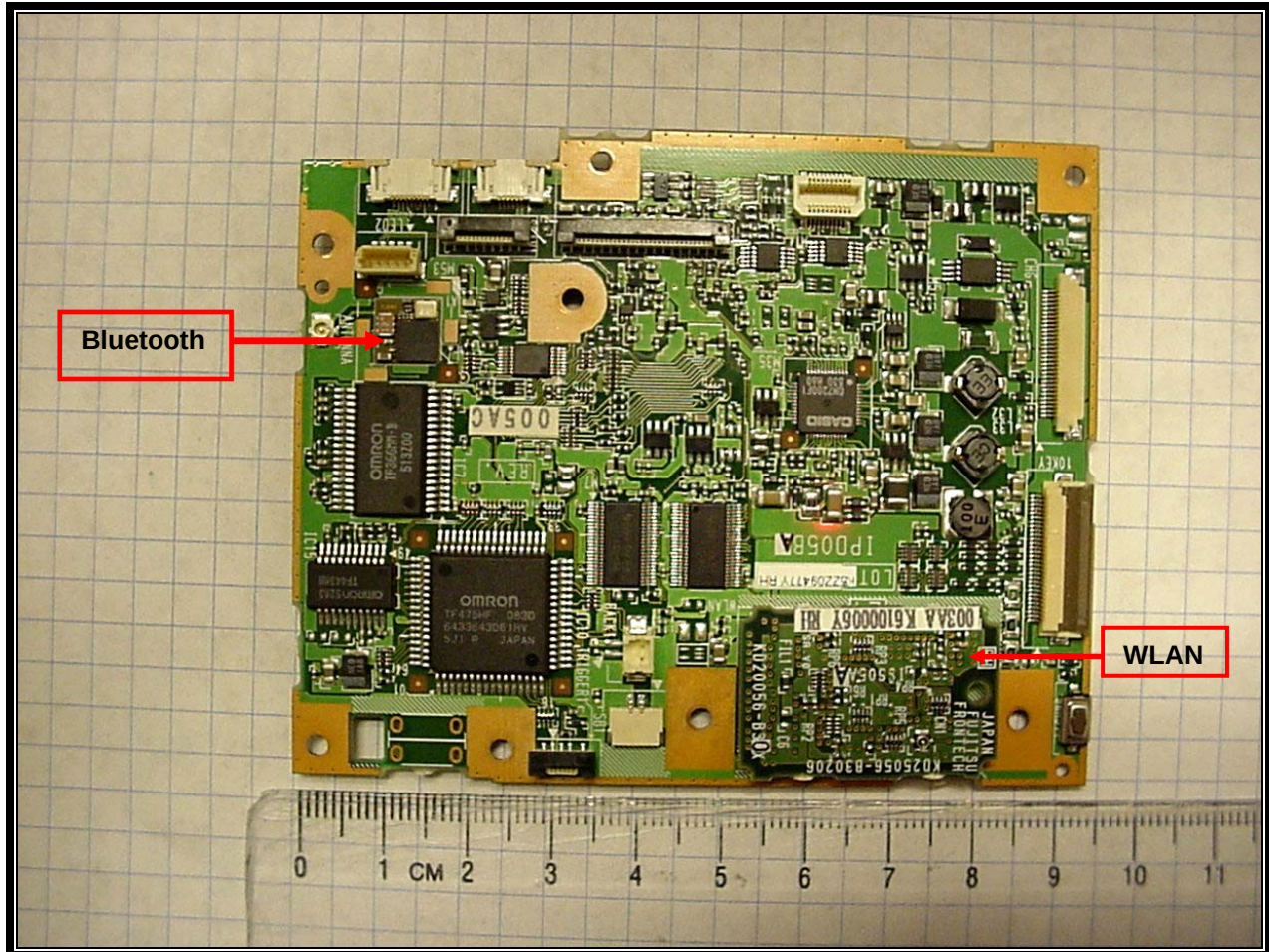
Photograph 13: Back Side of PCB with WLAN PCB Attached
