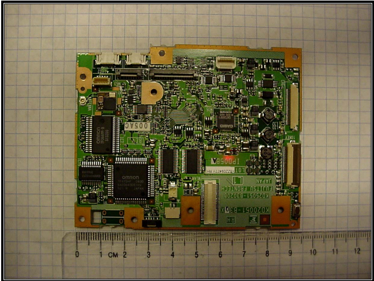
Photograph 14: Back Side of PCB with WLAN PCB Removed
