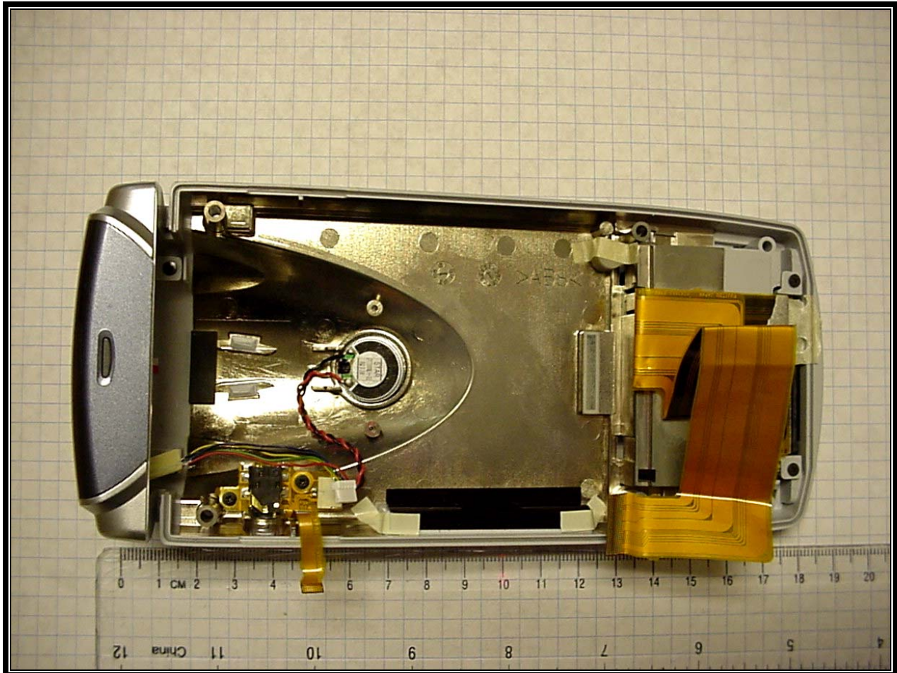
Photograph 11: Inside of Rear Case
