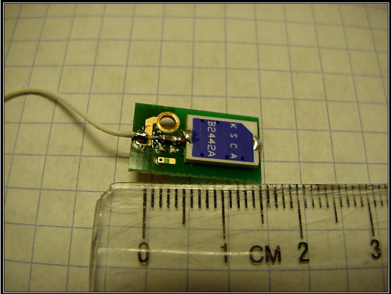
Photograph 24: Top of Bluetooth Antenna
