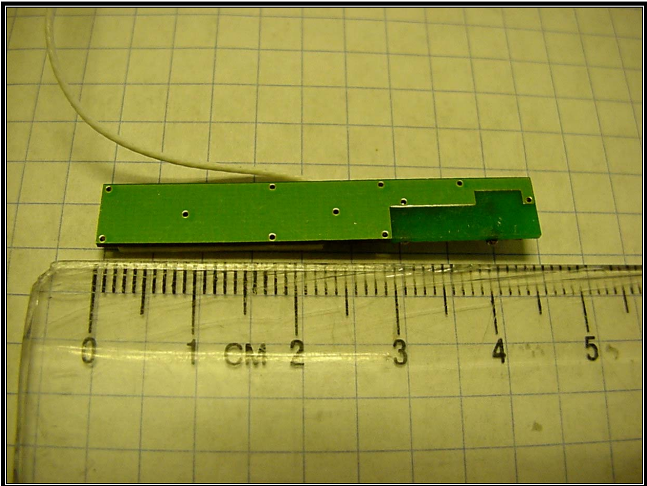
Photograph 19: WLAN Antenna - Back Side
