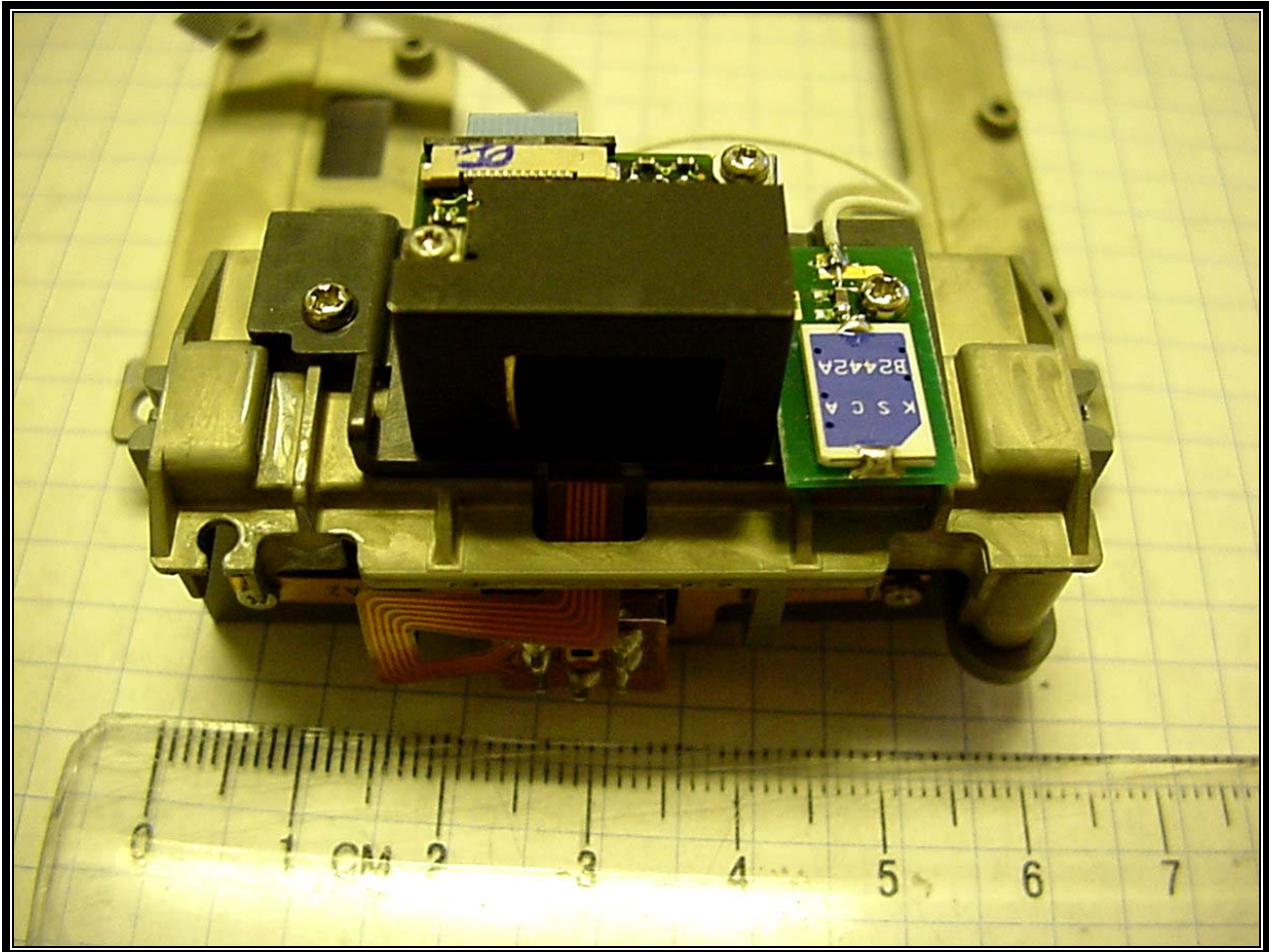
Photograph 27: Chassis Assembly with Bluetooth Antenna and Scanner
