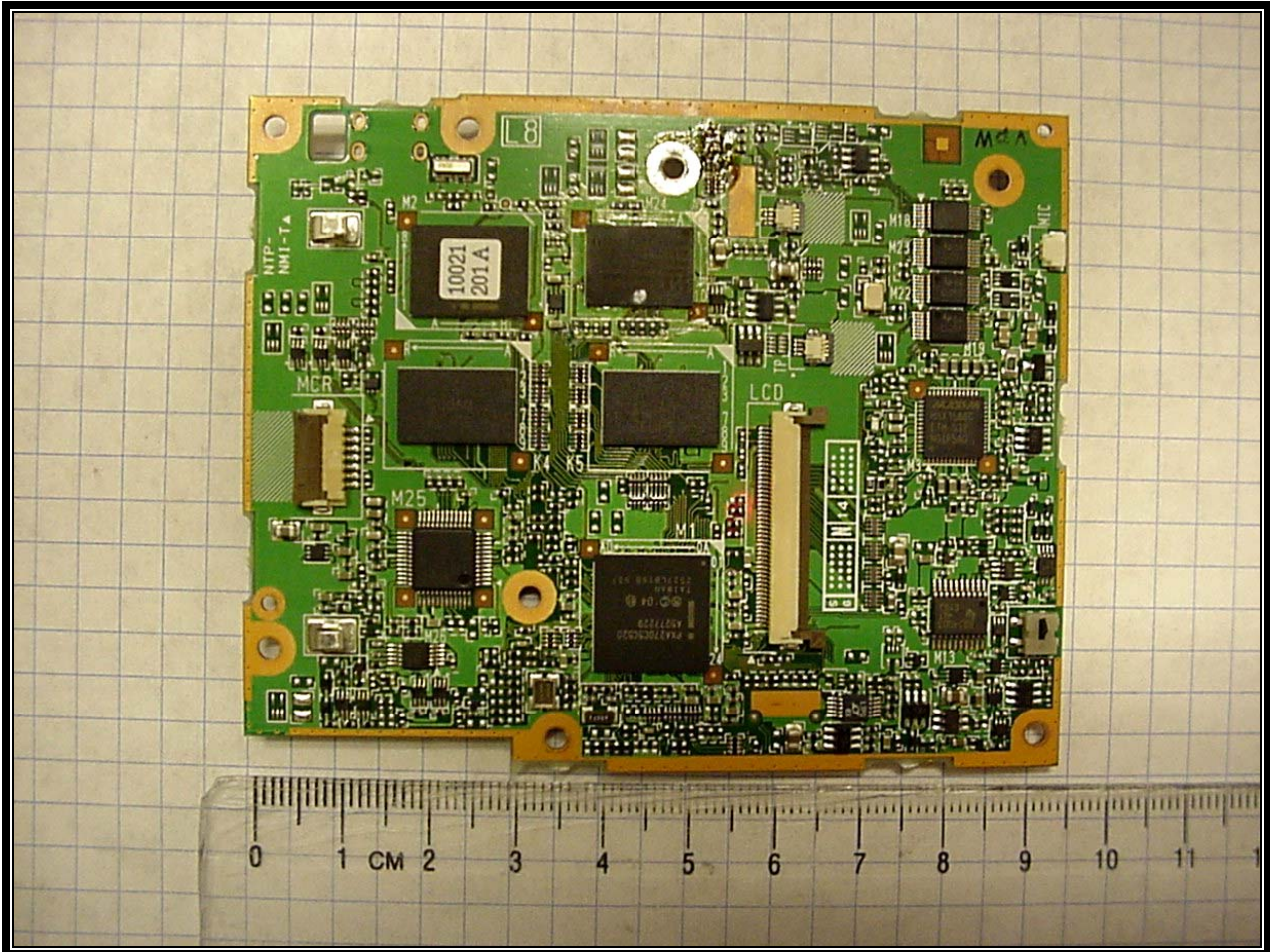
Photograph 12: PCB Front Side
