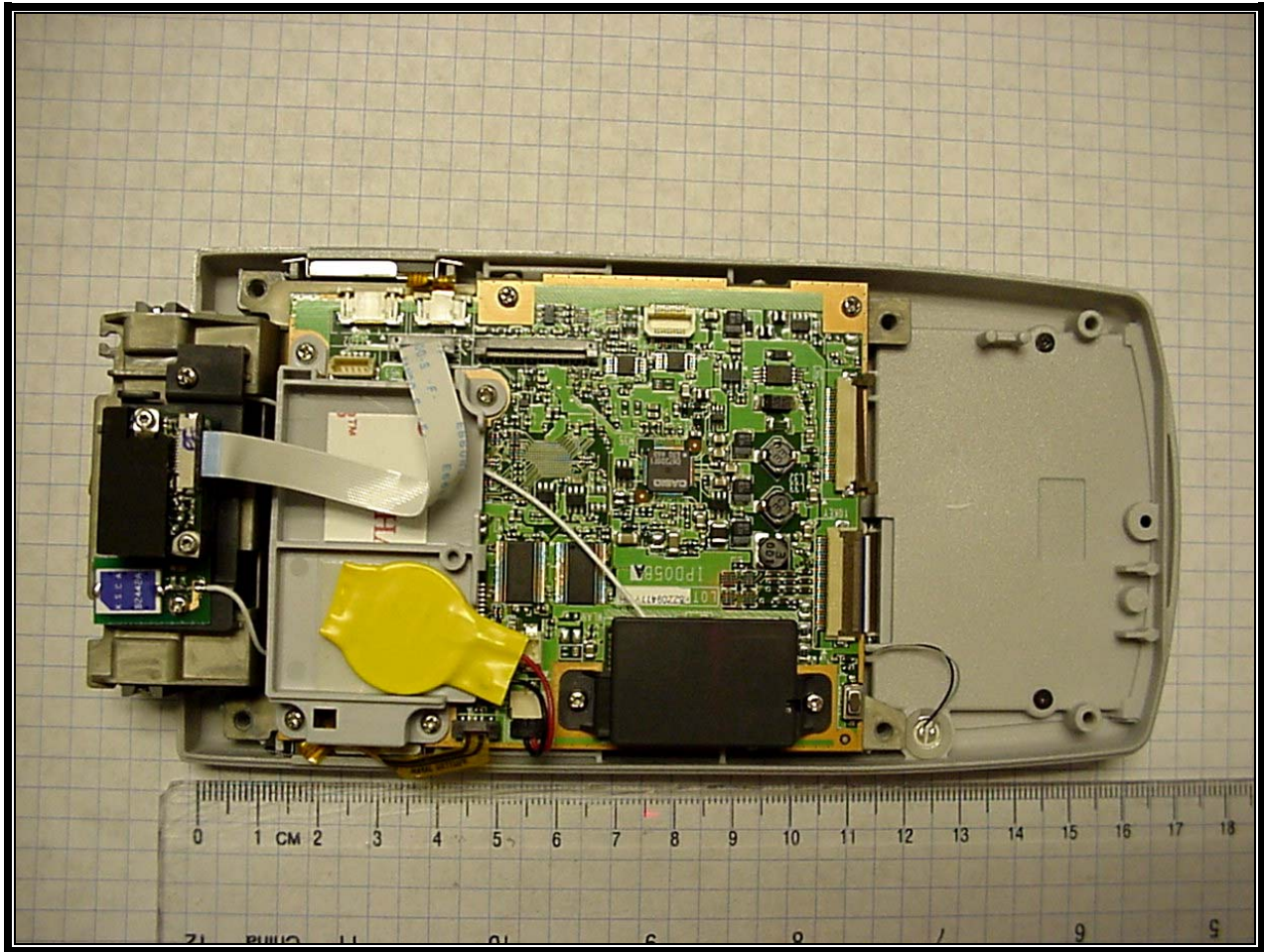
Photograph 10: PCB in Front Chassis
