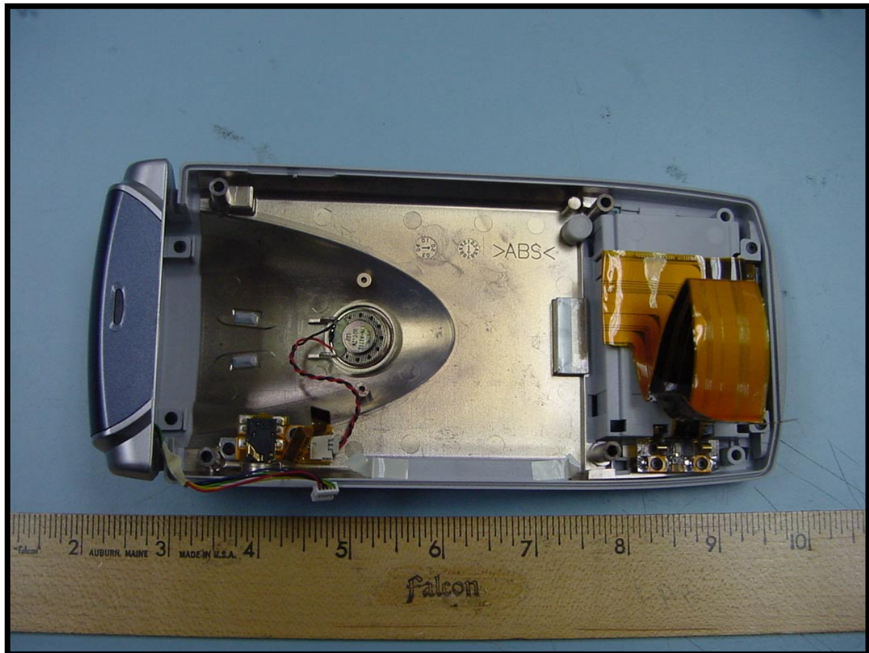
PHOTOGRAPH 25: INSIDE OF OTHER ENCLOSURE
