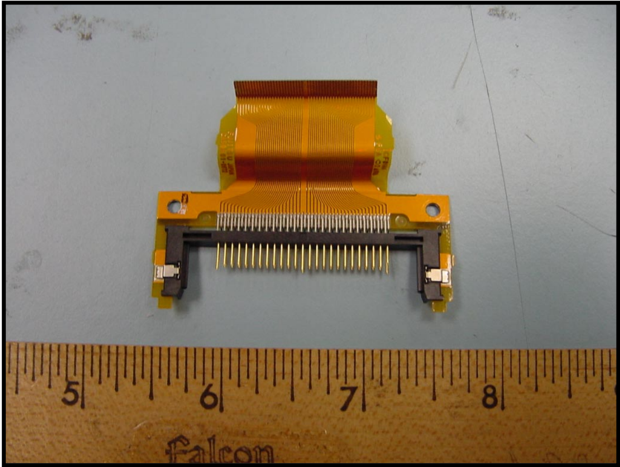
PHOTOGRAPH 19: INTERFACE CABLE
