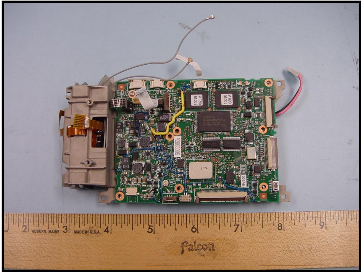
PHOTOGRAPH 12: MAIN PCB
