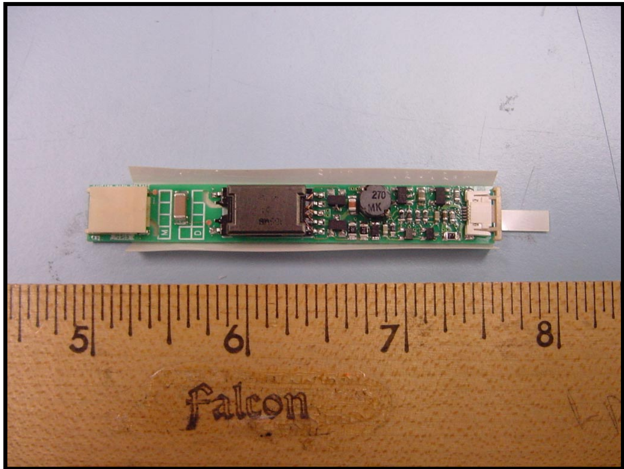
PHOTOGRAPH 18: INVERTER
