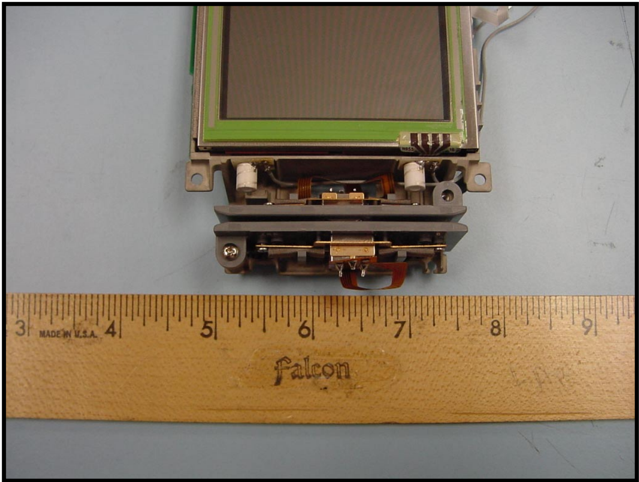
PHOTOGRAPH 14: DISPLAY
