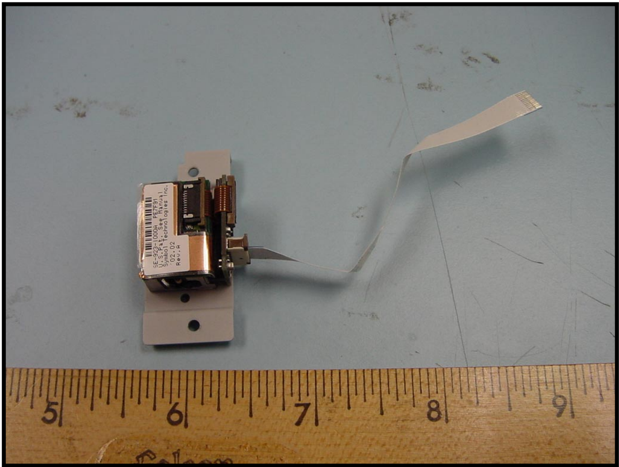
PHOTOGRAPH 21: SCANNER ENGINE
