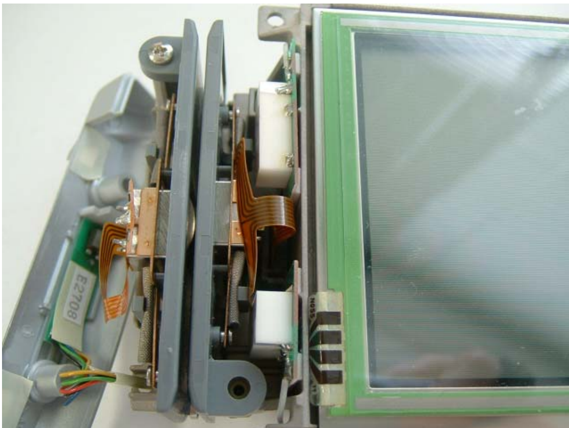
Enlarged view of Antenna (No.1)
