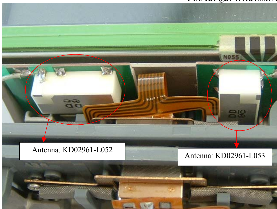
Enlarged view of Antenna (No. 2)
