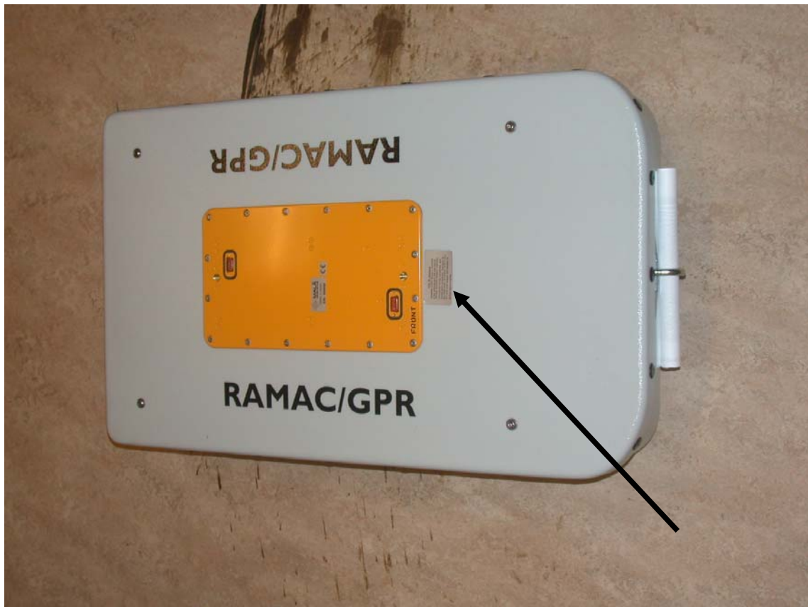
Figure 2. Placement of the FCC label on top-front of the UWB-unit, visible all times.
