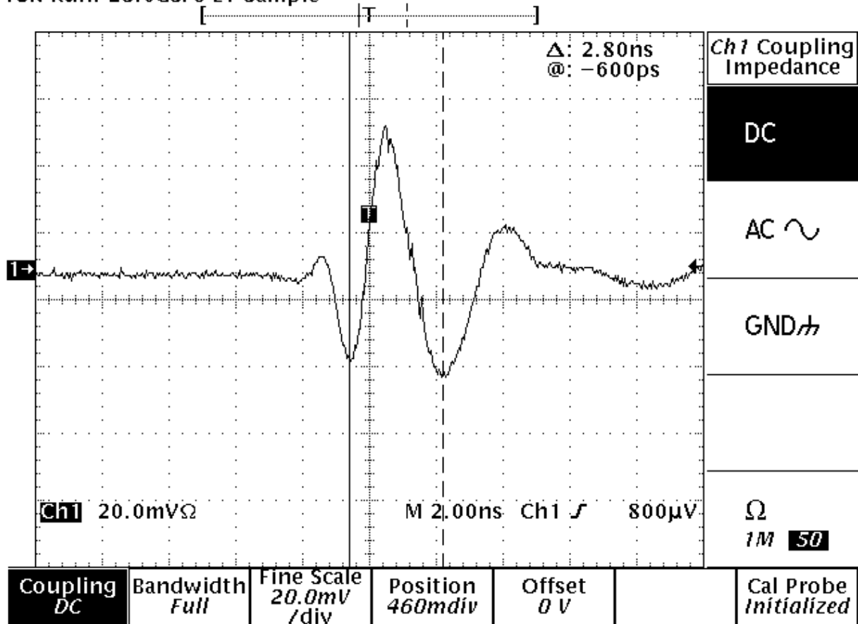
Figure 1. Pulse characteristic of a 250 UWB-unit.
